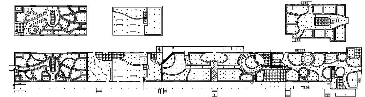
Building RCP
