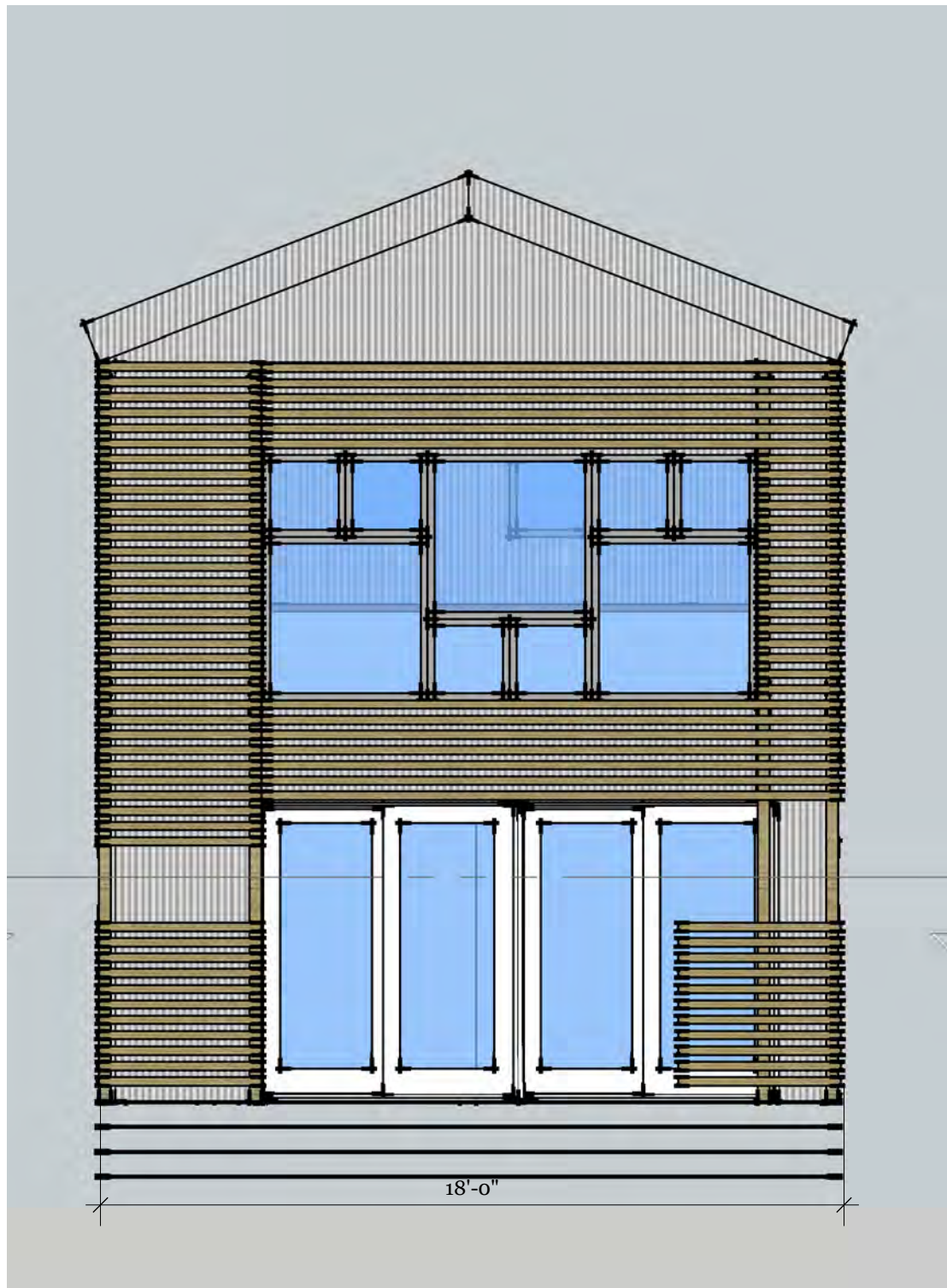
FRONT VIEW scale: 1/4"=1'
