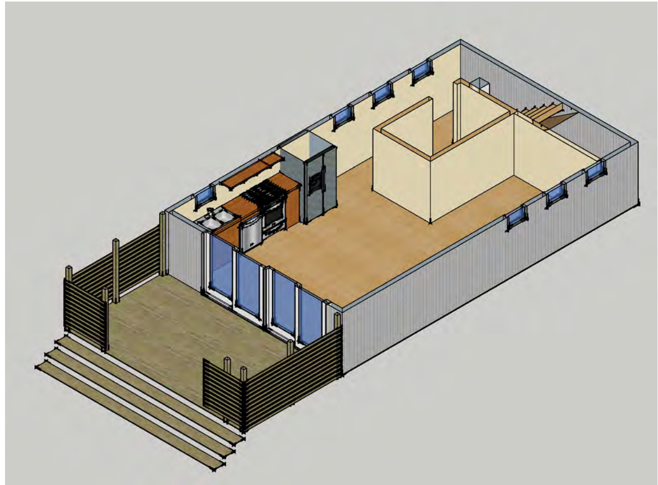
ISOMETRIC VIEW scale: 1/8"=1'
