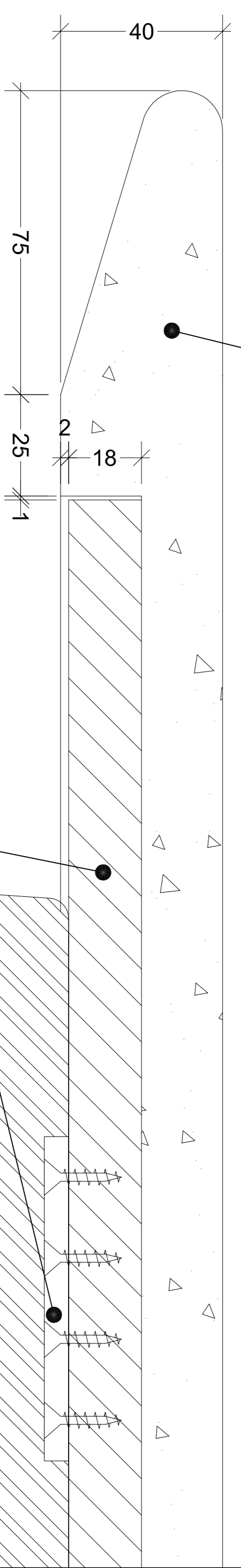
TOP BONDED TO 18MM MDF PANEL AND SCREWED FROM BELOW
