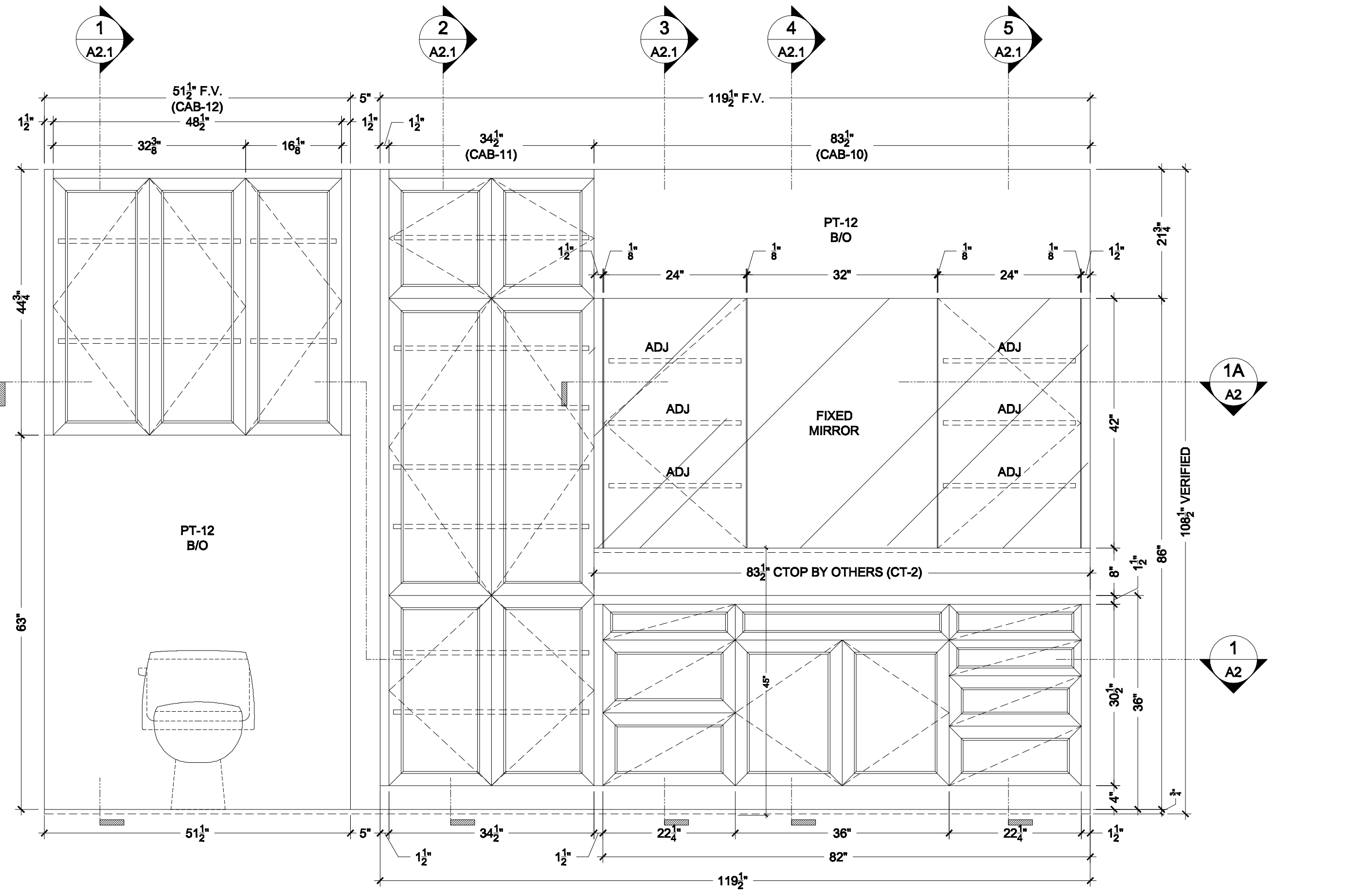
2 WC 3 SCALE: 3/4" = 1'-0" REF: CAB-12 FINISH:
