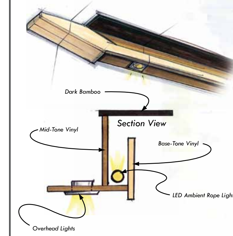
Light Valance Detail
