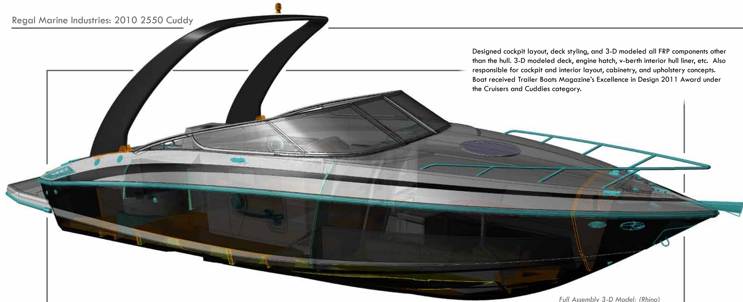
Full Assembly 3-D Model: (Rhino)
