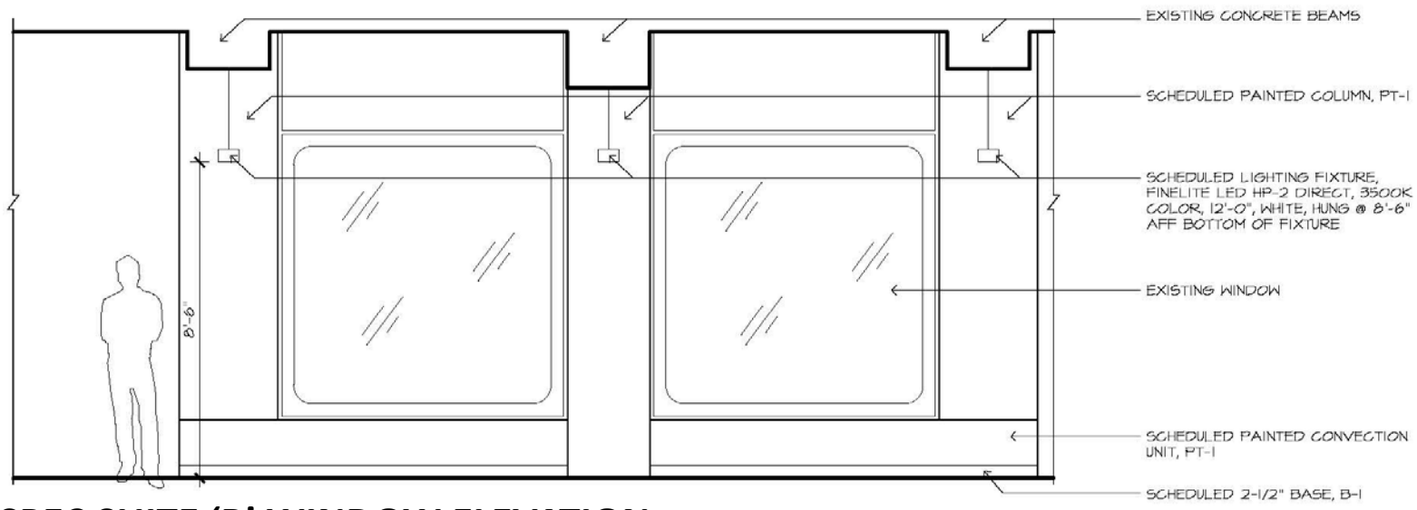
SPEC SUITE 'B' WINDOW ELEVATION
