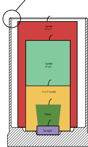
Section view with candles in holder
