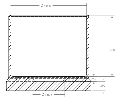
Section View
