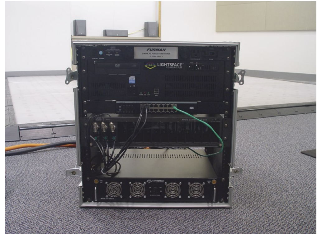
3 Photo of Lightspace Component Rack; Front for reference only
