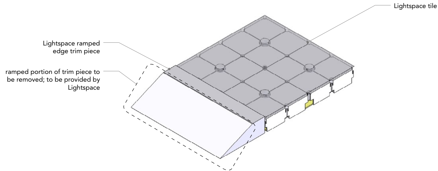
1 Detail; Lightspace Panel scale: NTS
