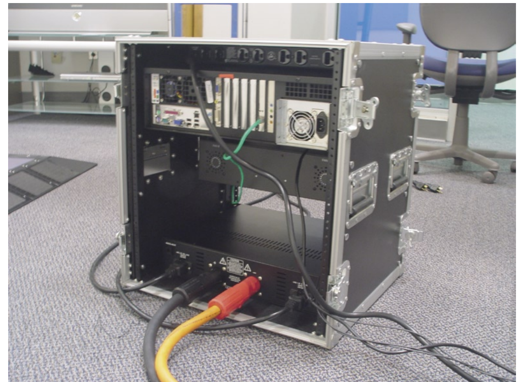
4 Photo of Lightspace Component Rack; Back for reference only
