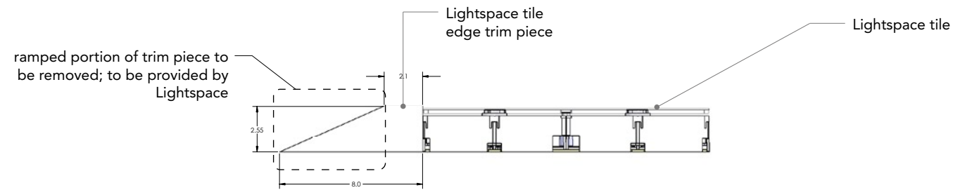
2 Detail; Lightspace Panel scale: NTS
