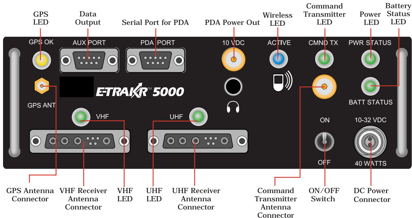
E-TRAK/R-5000 Front Panel Connections
