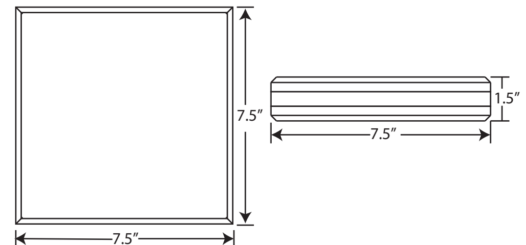
Basic Dimensions
