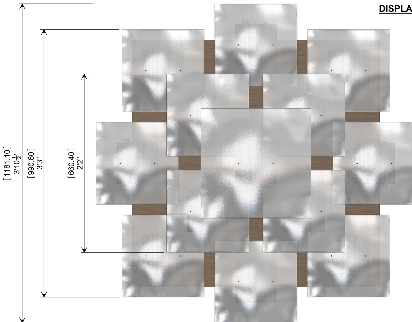
REFLECTED PLAN VIEW
