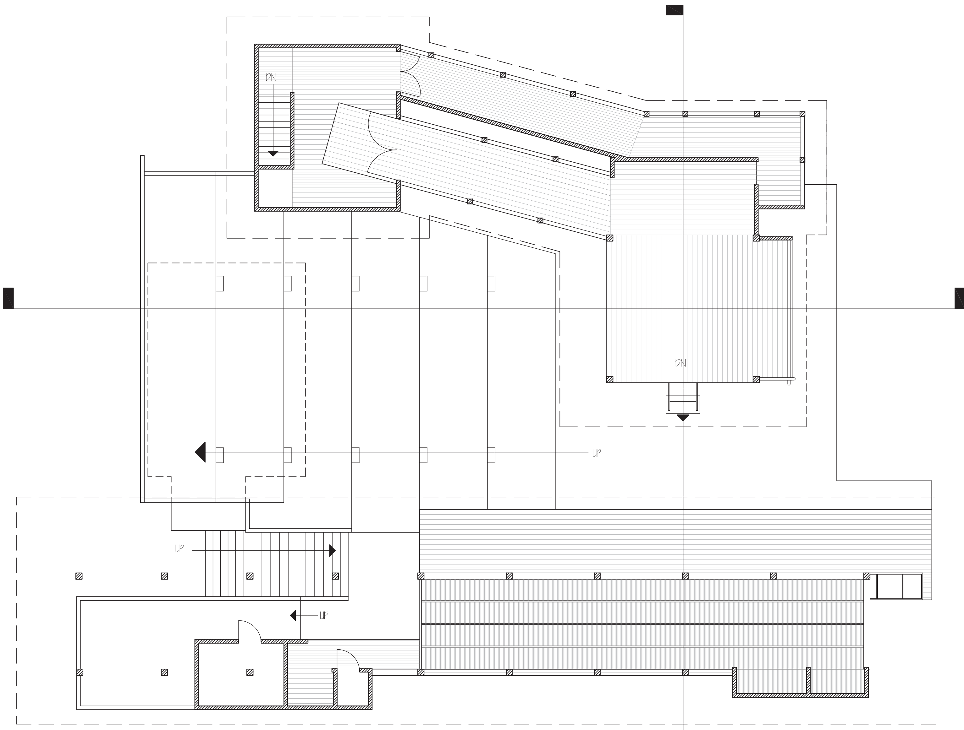
FLOOR PLAN 1/8"=1'-0" 0" 8"
