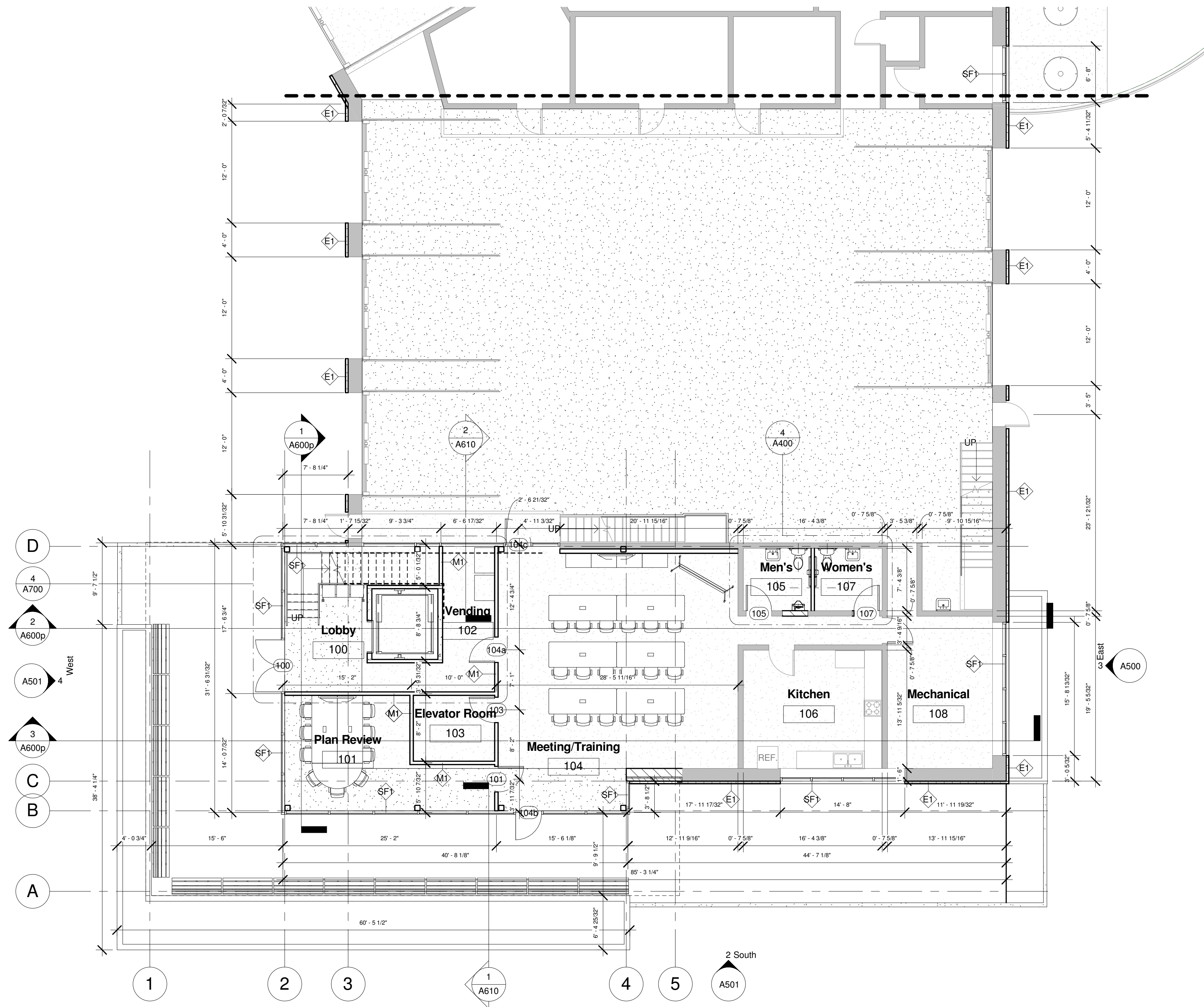
1 Main Level (South) 1/8" = 1'-0"
