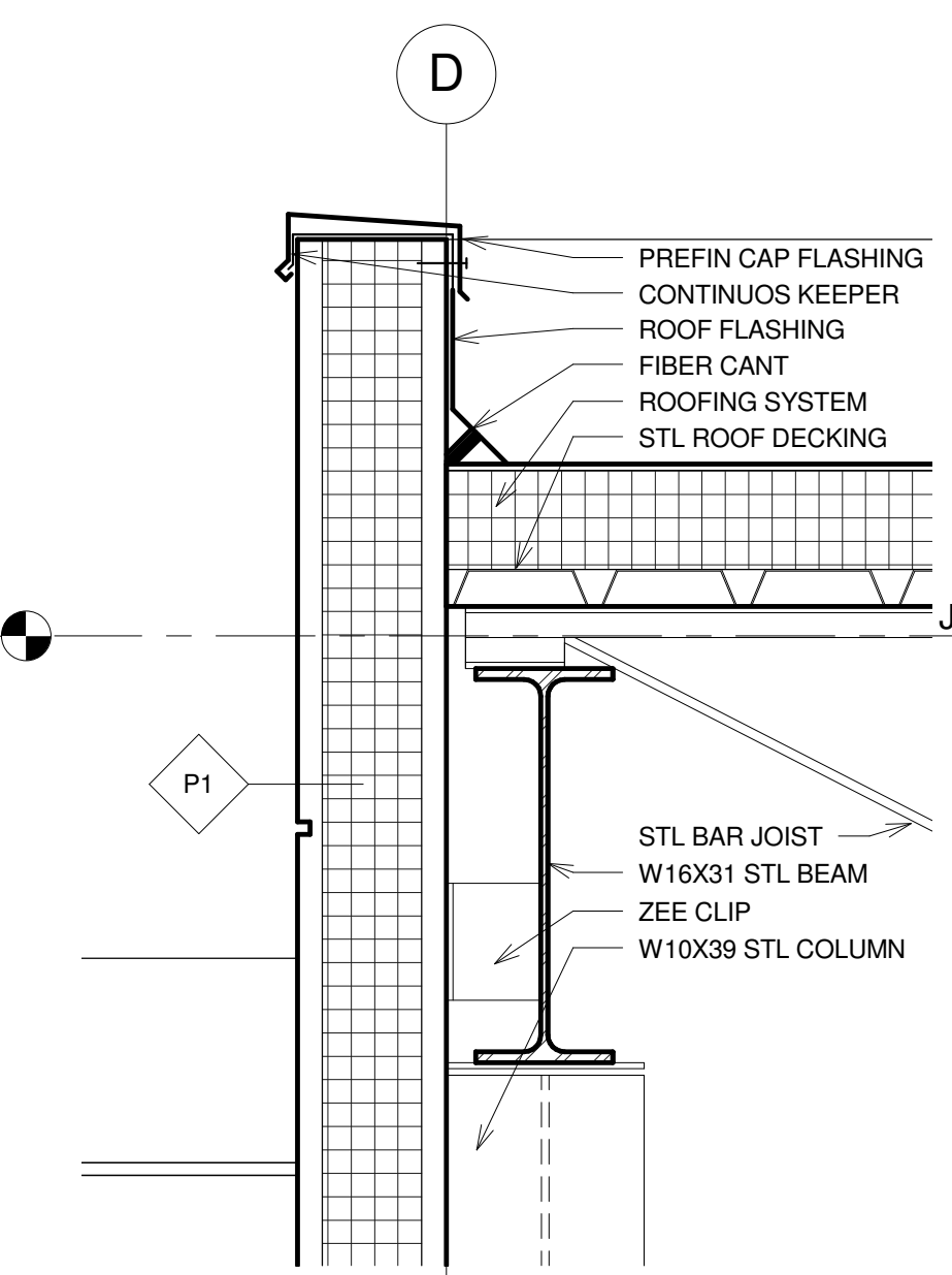
3 Roof Edge Perpendicular To Structure 1 1/2" = 1'-0"
