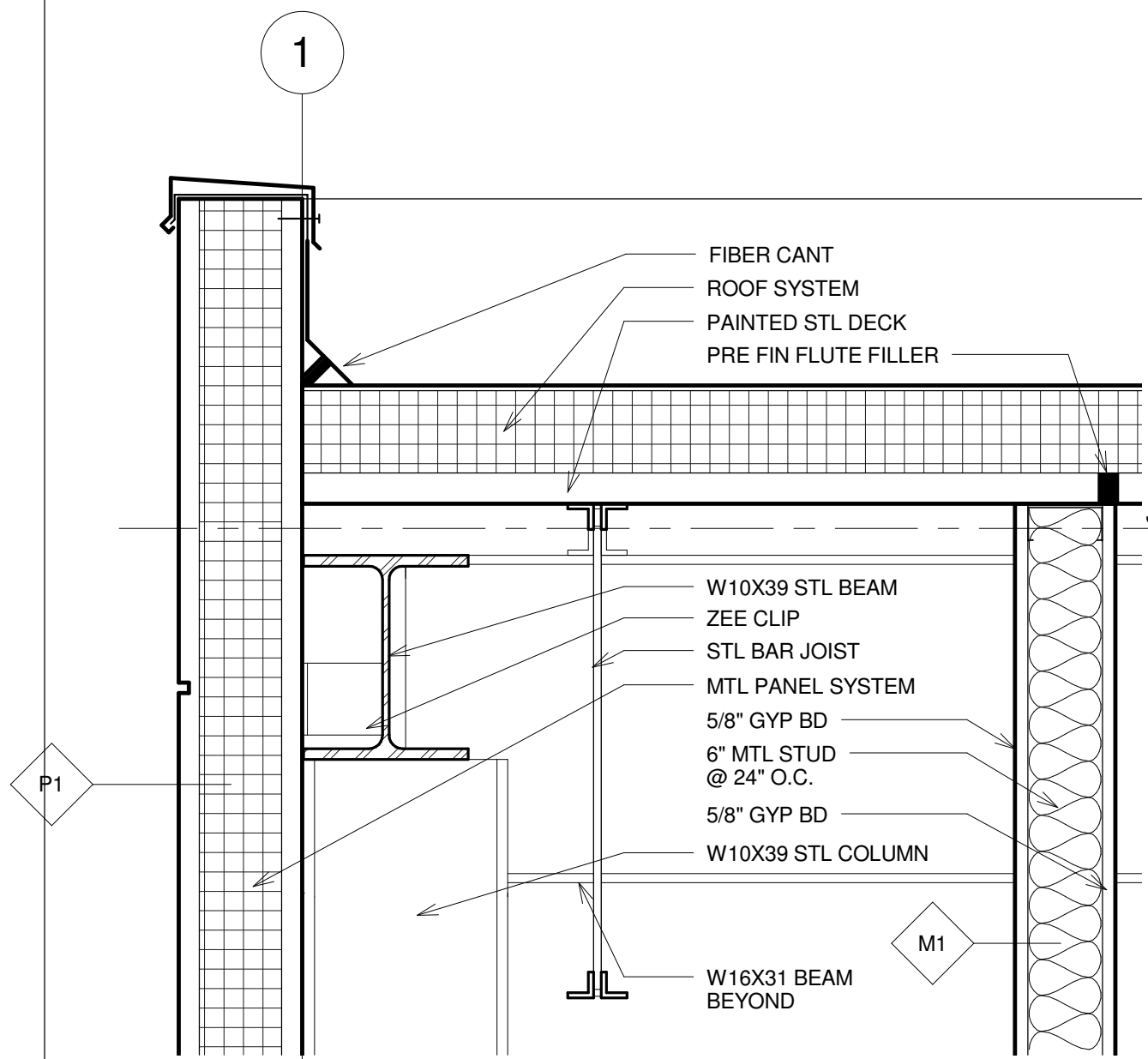
5 Roof Edge @ Bay Window 1 1/2" = 1'-0"
