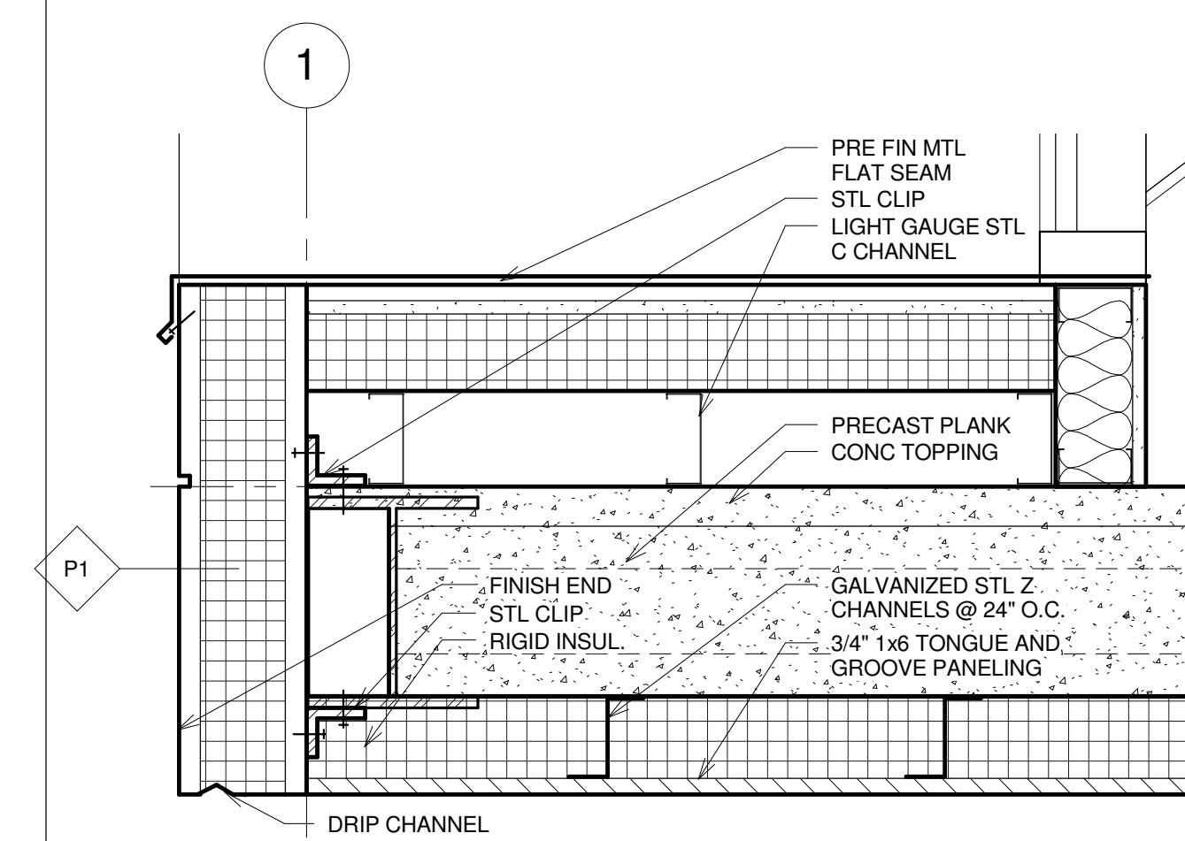
4 Plank Edge Detail @ Entry 1 1/2" = 1'-0"
