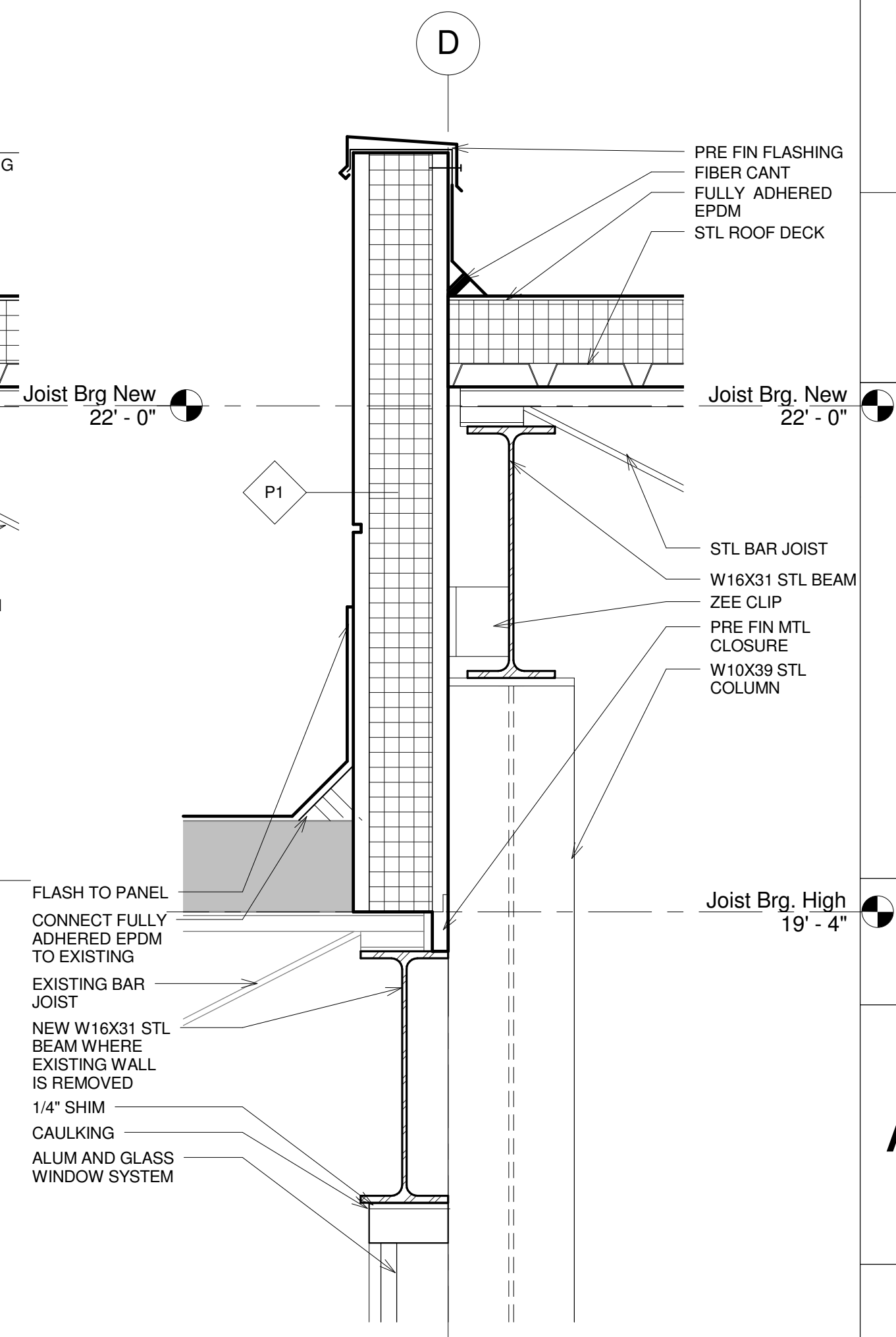
2 High/Low Roof Connection 1 1/2" = 1'-0"
