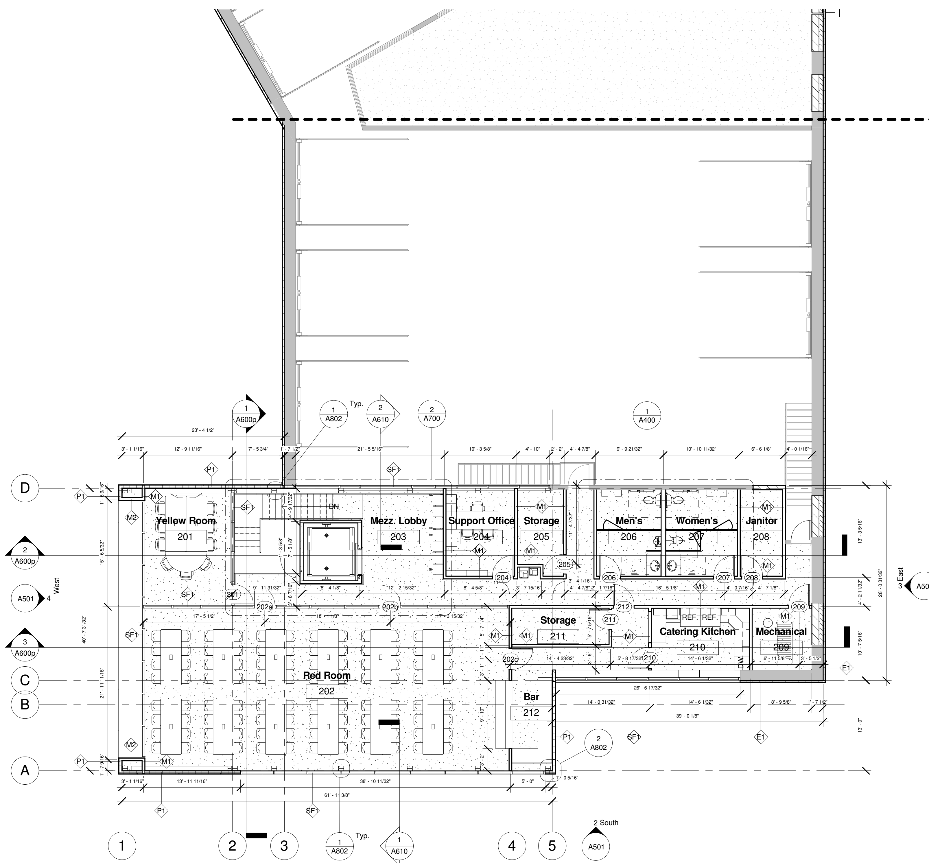
1 Mezzanine Plan (South) 1/8" = 1'-0"
