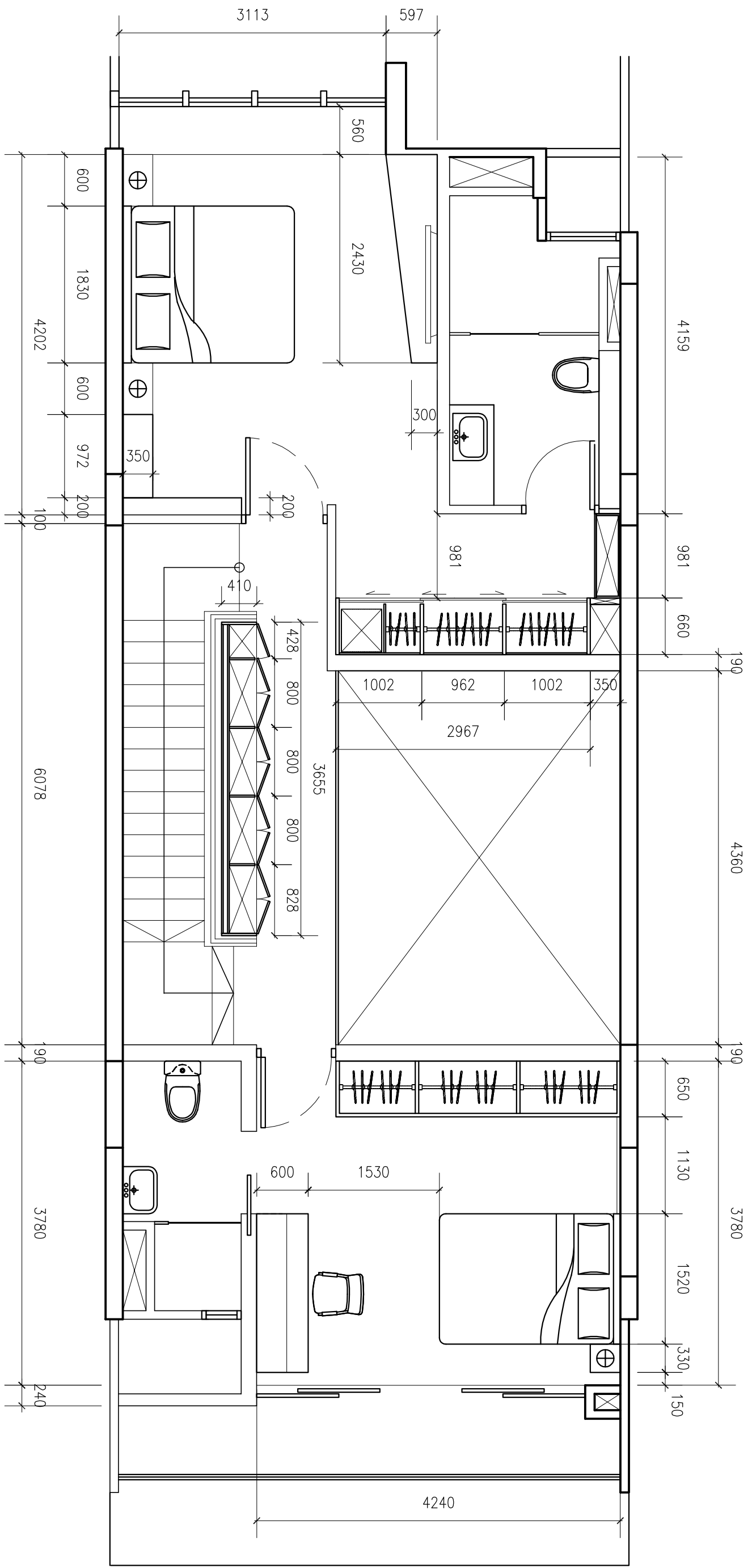
2nd STOREY - LAYOUT PLAN SCALE 1:50
