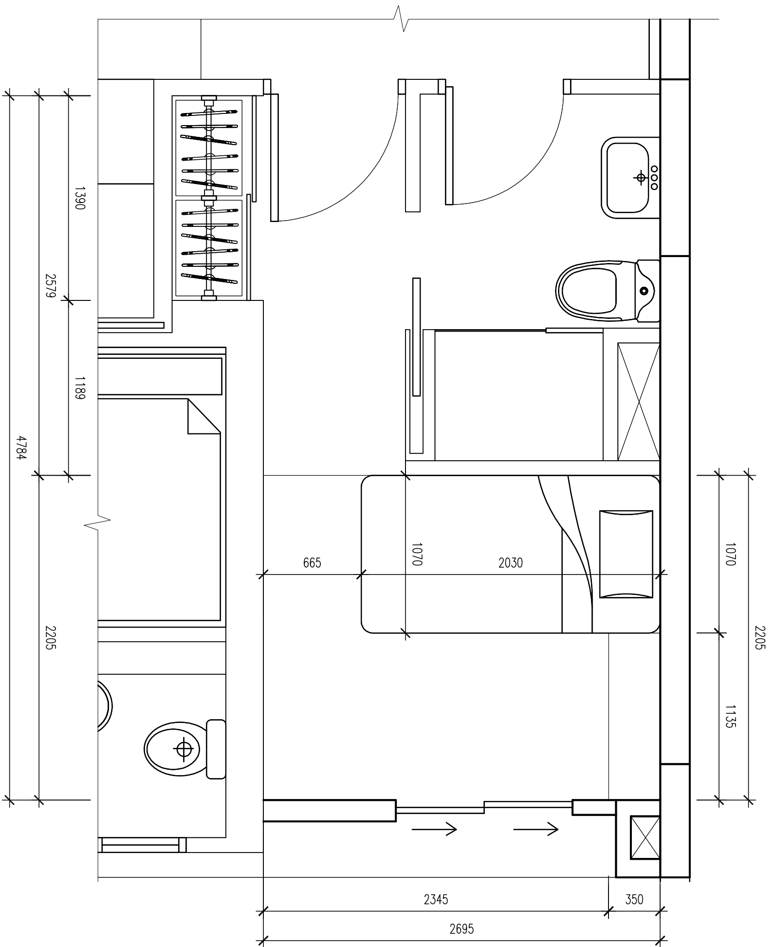
MOM'S BEDROOM - LAYOUT PLAN SCALE 1:25
