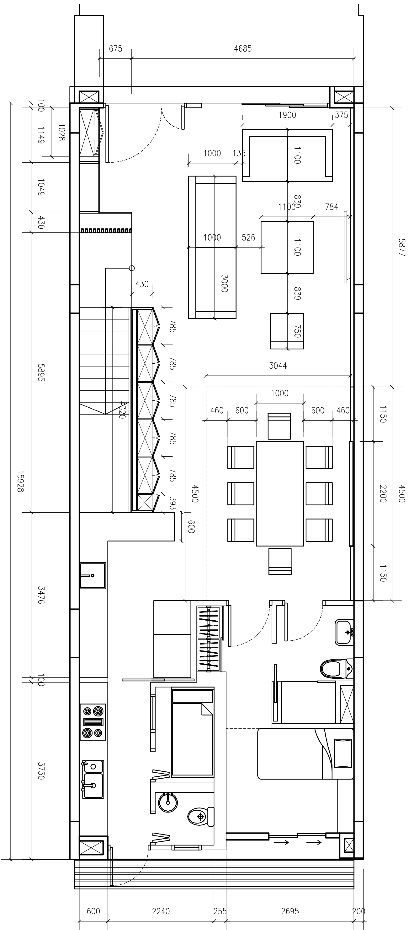
1st STOREY - LAYOUT PLAN SCALE 1:50
