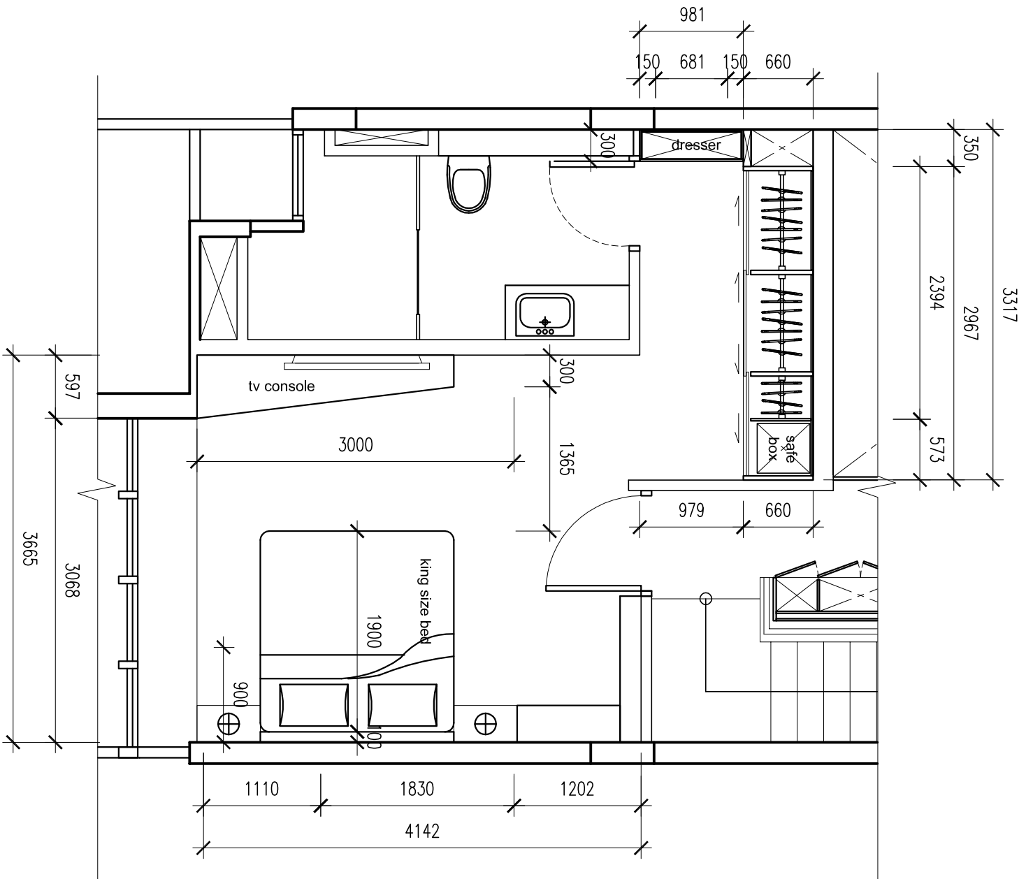
MASTER BEDROOM - LAY OUT PLAN SCALE 1:25
