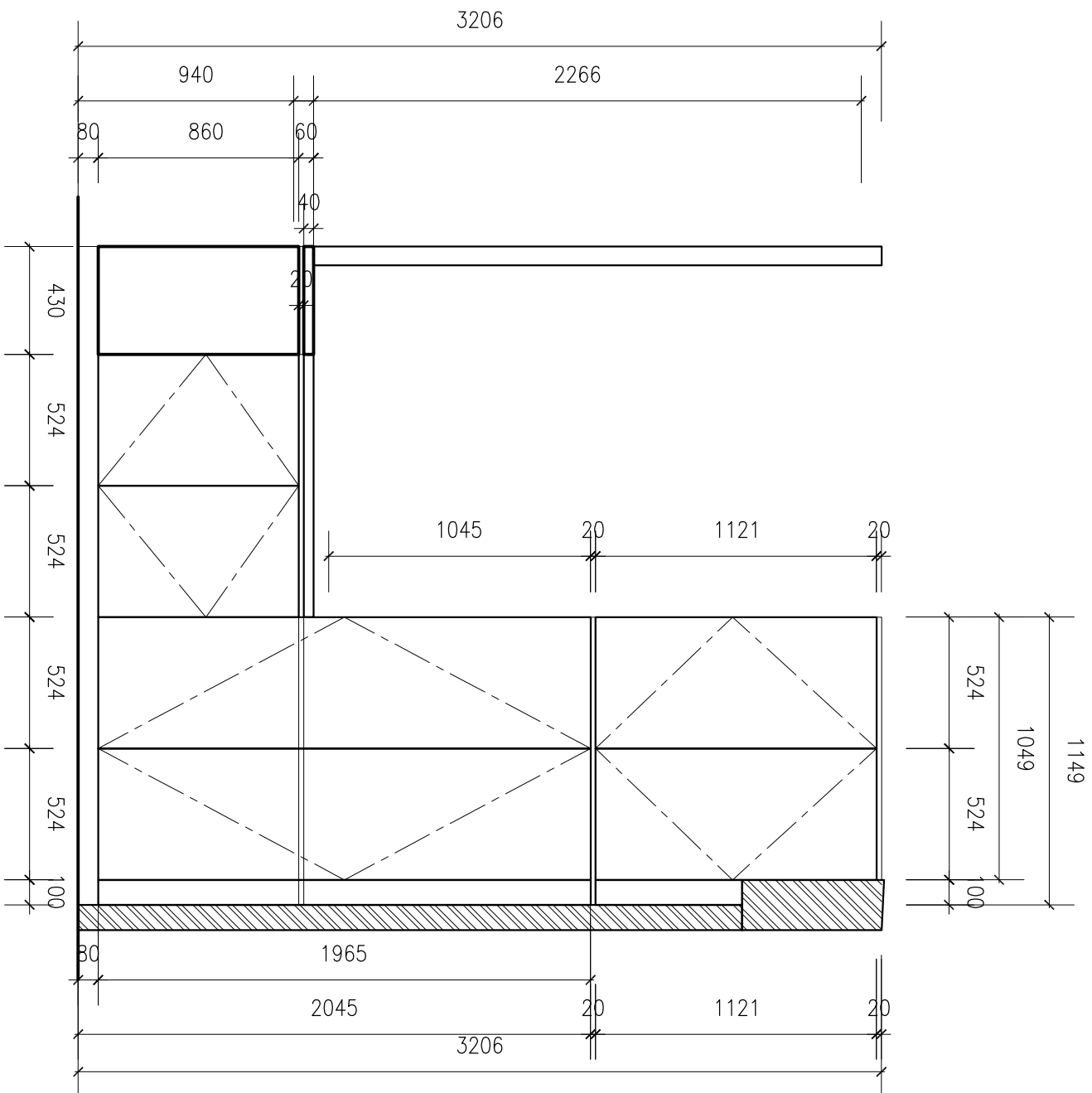
DB CABINET - ELEVATION 4 SCALE 1:25
