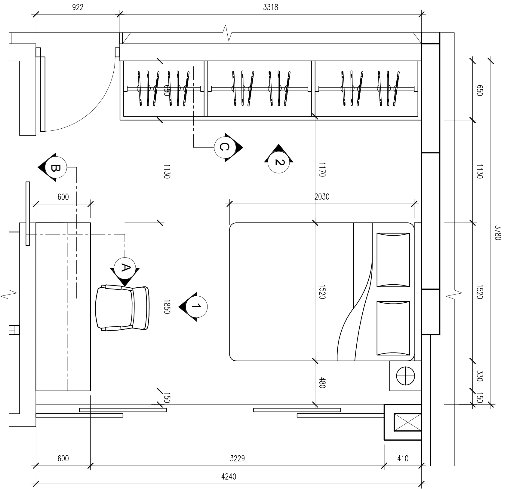
DAUGHTER BEDROOM - LAY OUT PLAN SCALE 1:25
