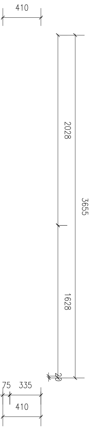
CORRIDOR CABINET - TOP ELEVATION SCALE 1:25
