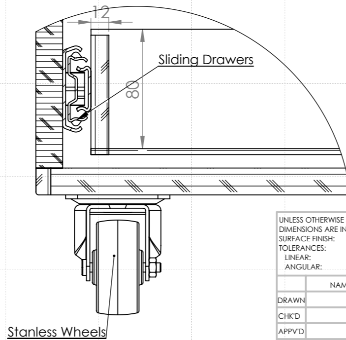
DETAIL H SCALE 2 : 5
