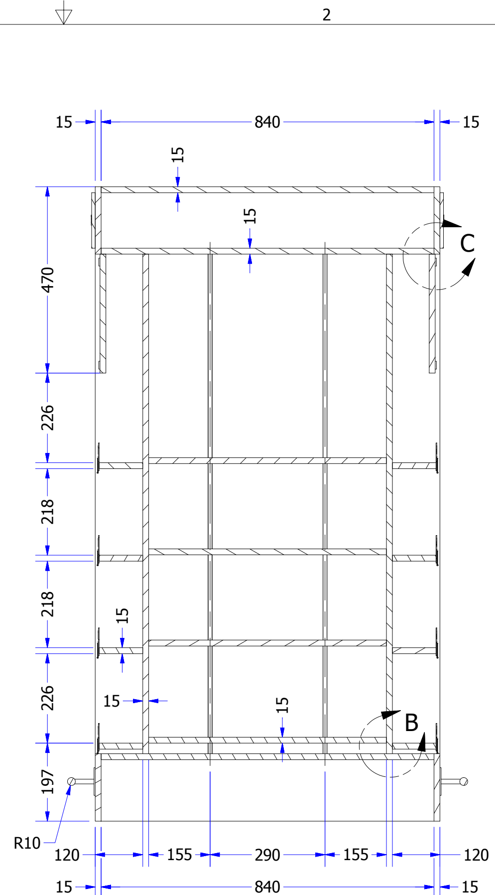
SECTION A-A SCALE 1 : 9.5
