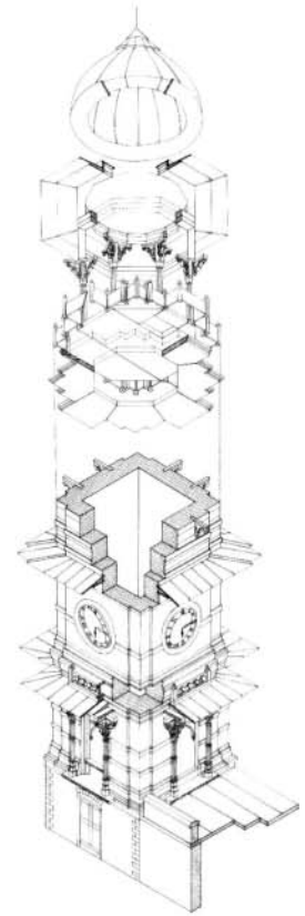
Isometric View of Clocktower
