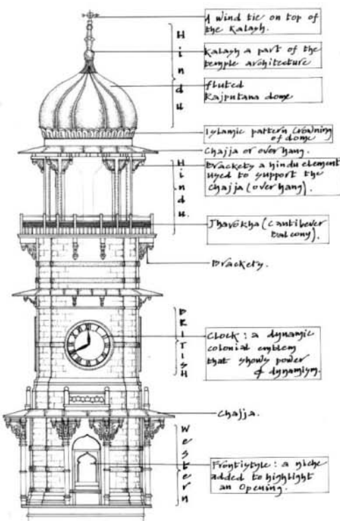
Elevation Of Clock Tower
