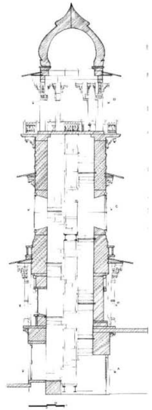
Section Through Clock Tower
