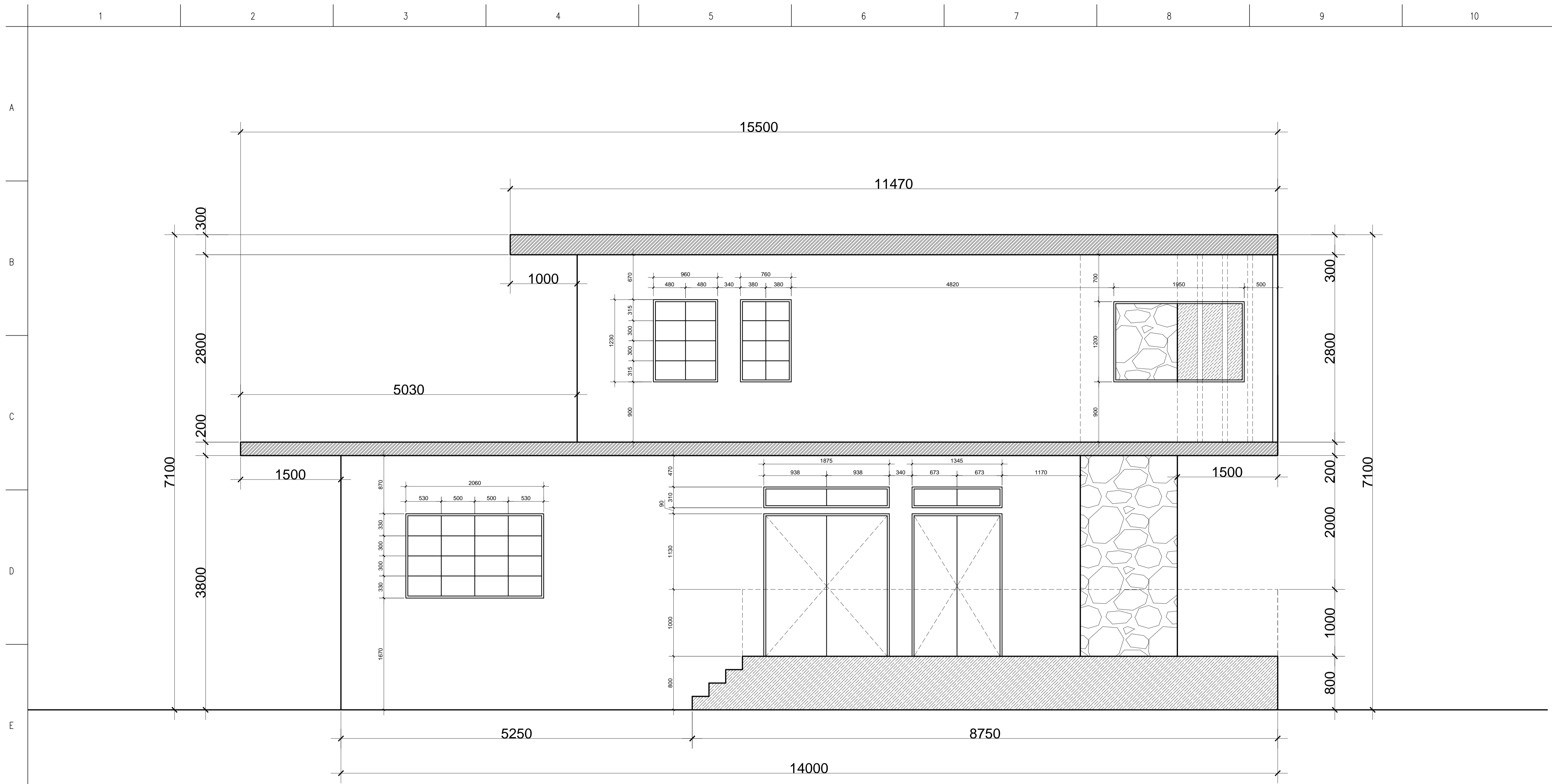
A ELEVATION B S-2 SCALE: 1:30 MTS.
