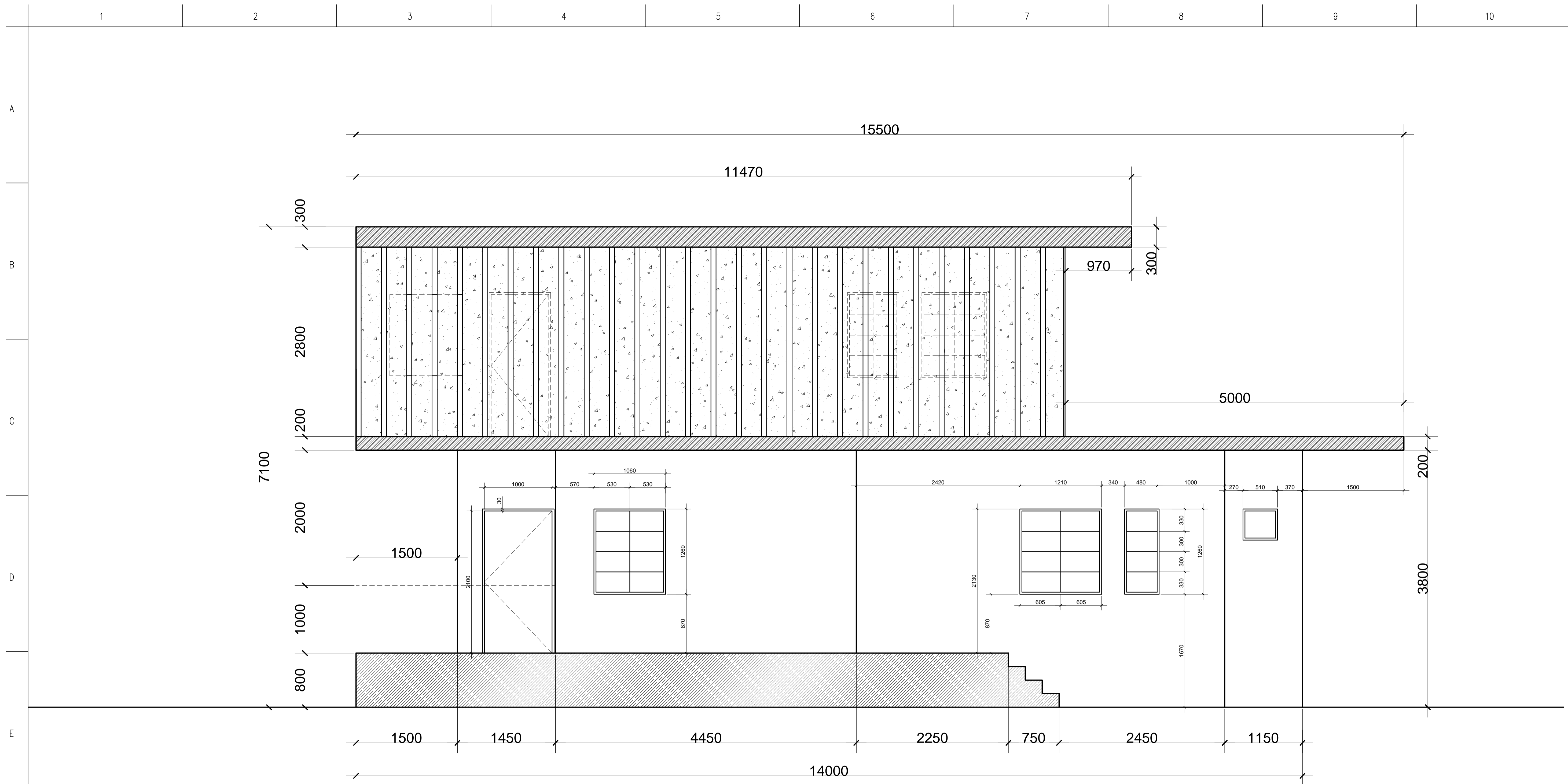
A ELEVATION C S-2 SCALE: 1:30 MTS.
