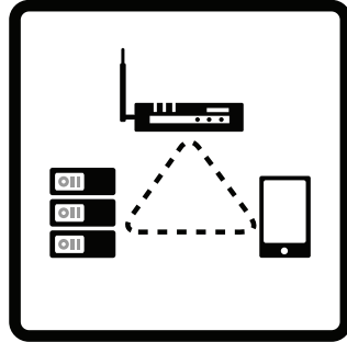
Clustering
