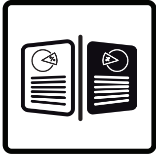
Replication
