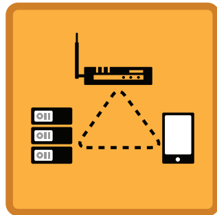
Clustering
