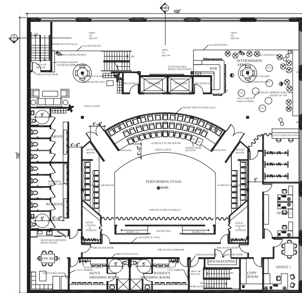
Metropolis 2nd Floor Plan Scale: NTS
