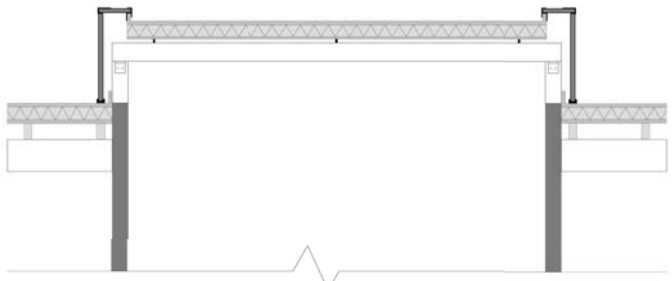
Detail Section of Ceiling
