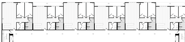
Typical two-bedroom, single-story apartment unit
