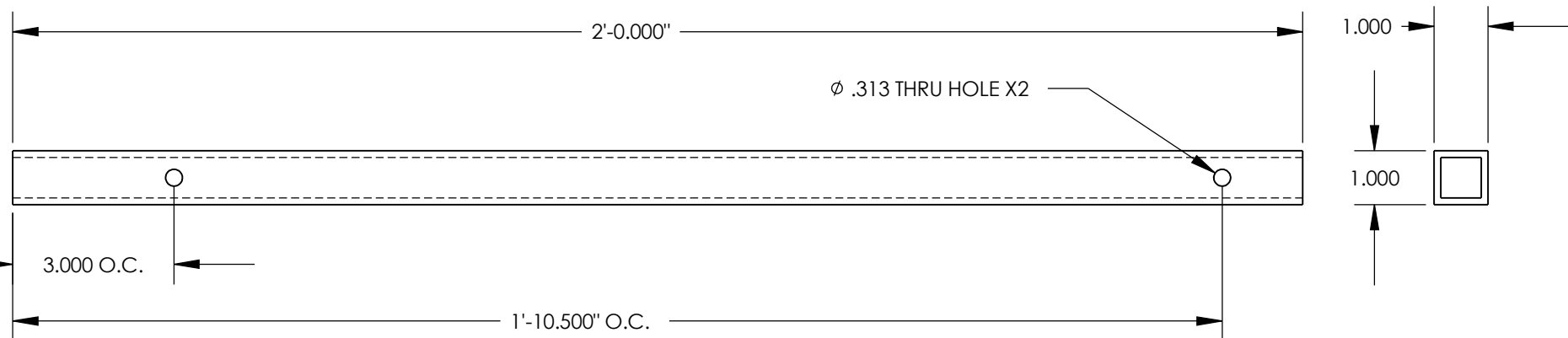
MATERIAL: 1" SQUARE TUBE
