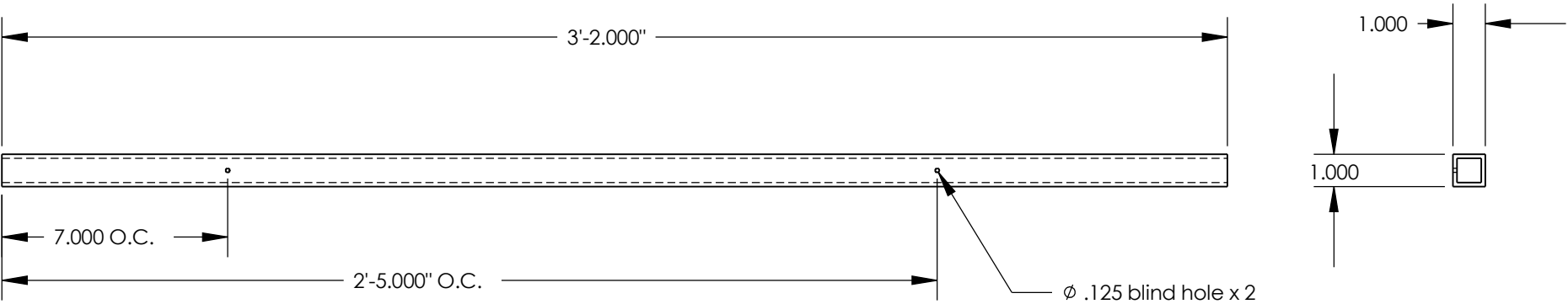
MATERIAL: 1" SQUARE TUBE
