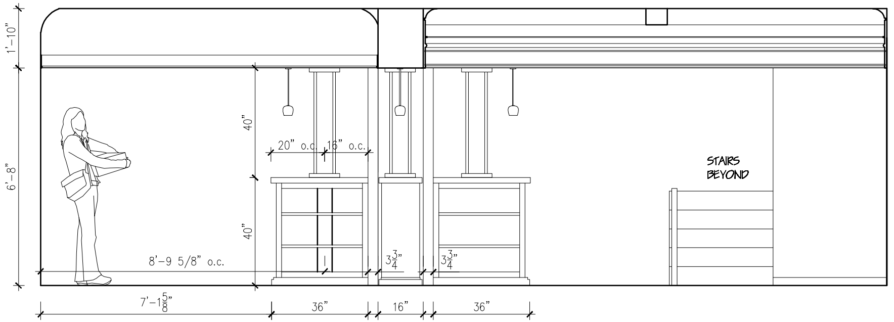
LIVING AREA ELEVATION
