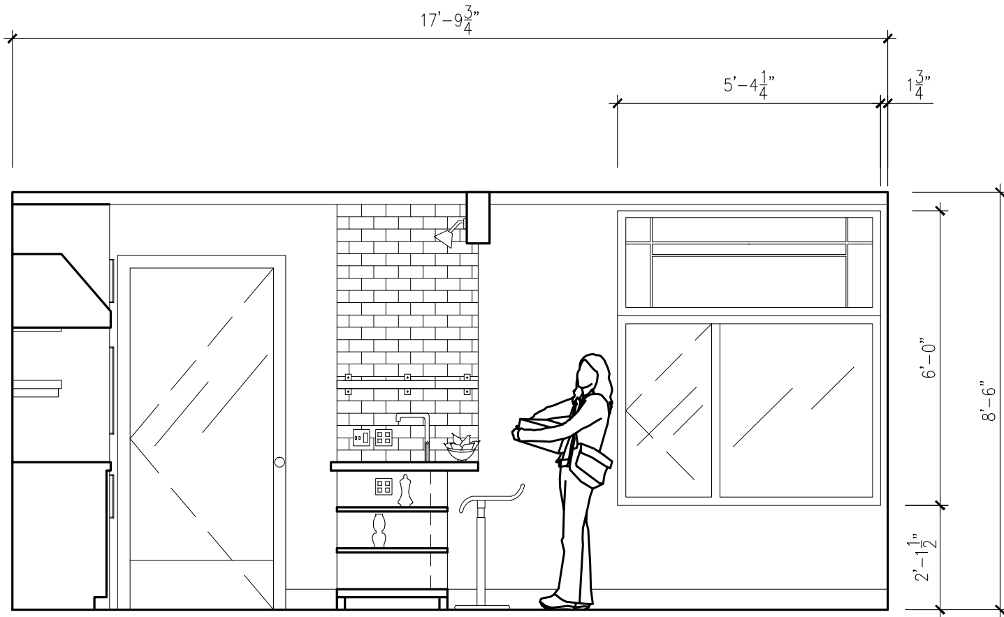
KITCHEN EAST ELEVATION
