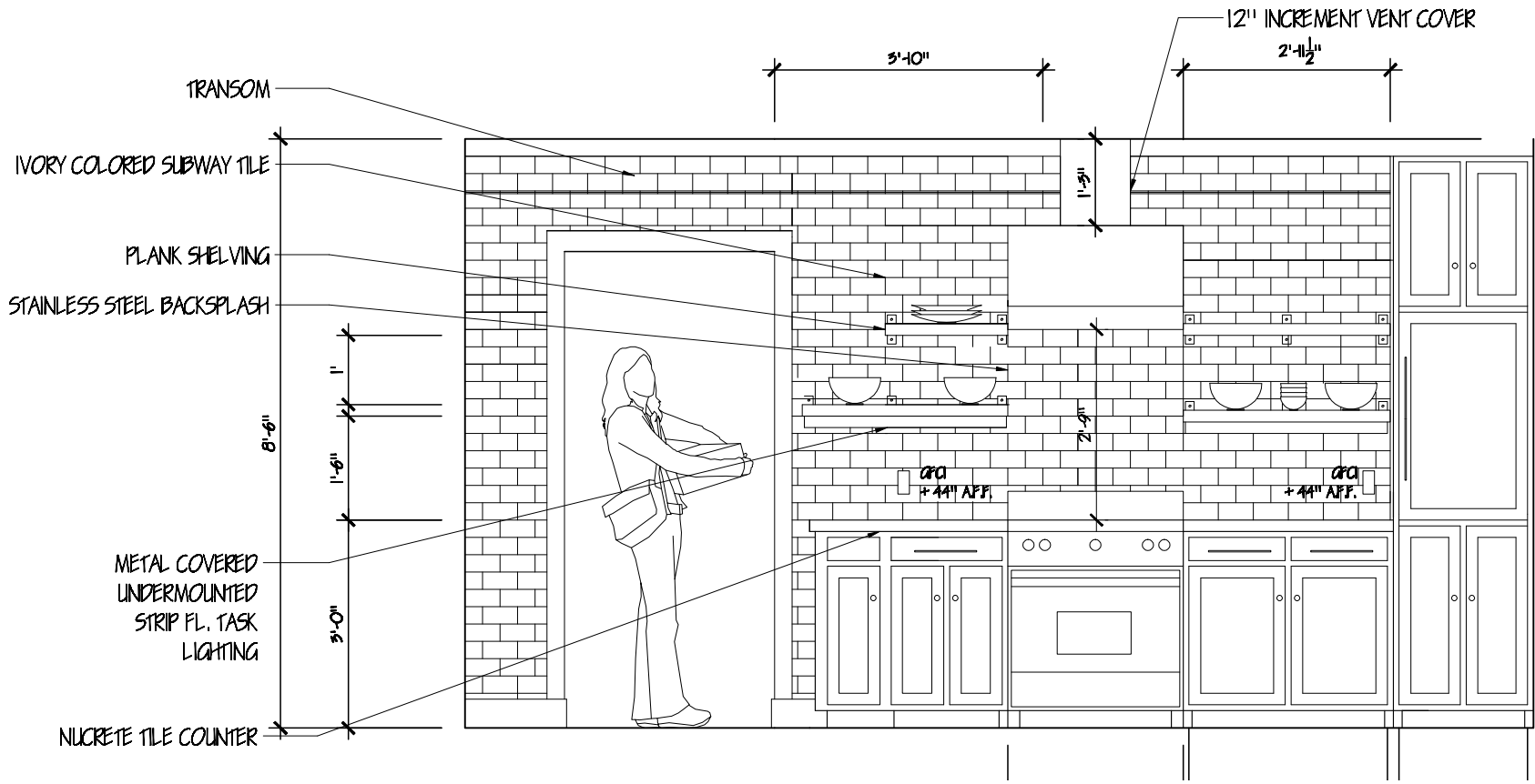
KITCHEN NORTH ELEVATION
