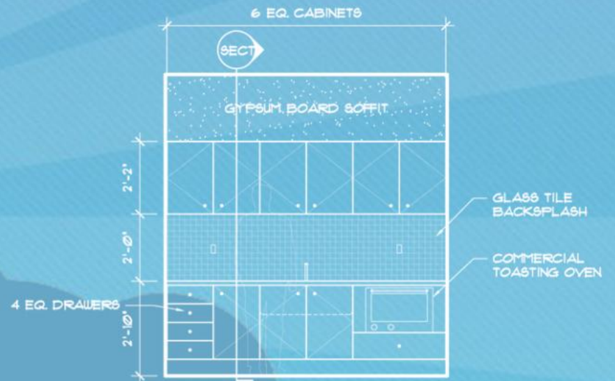
NOTE: ALL CABINETS TO BE LOCKING ELEVATION B
