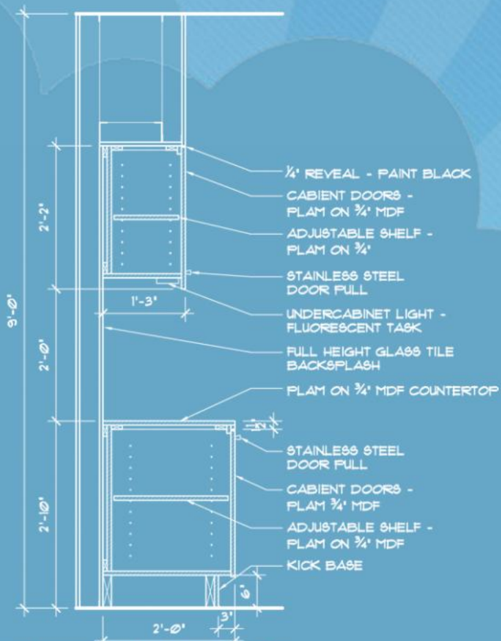
SANDWICH SHOP CABINET DETAIL 1/2"=1'-0"
