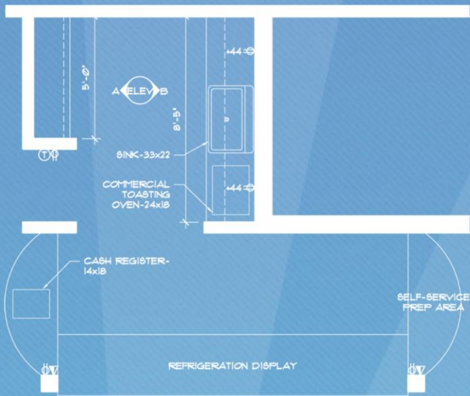
SANDWICH SHOP PREP COUNTER PLAN 1/4"=1'-0"
