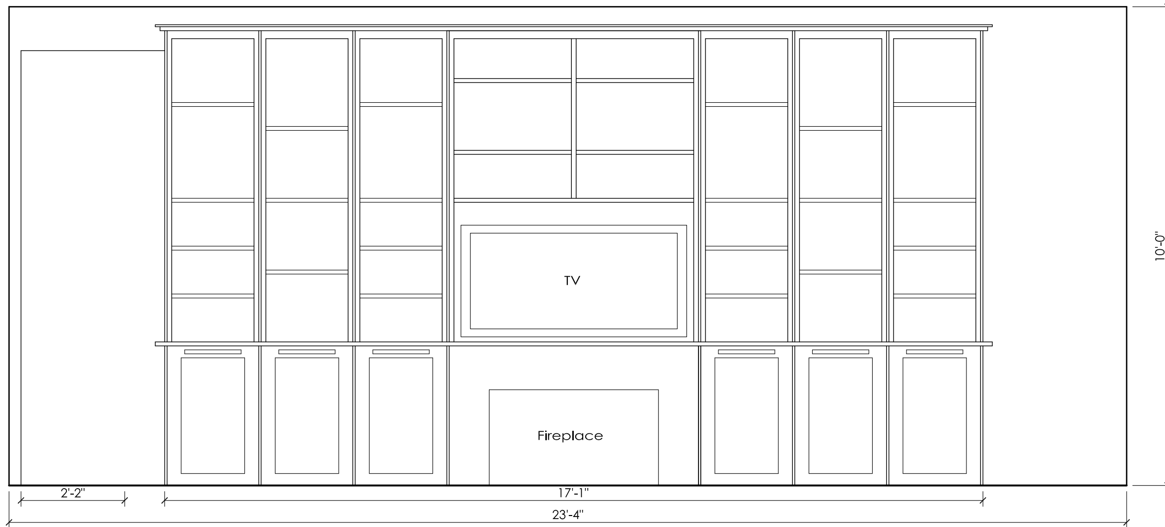
1 Living Room TV Wall Elevation Scale: \frac{1}{2} " = 1'-0"
