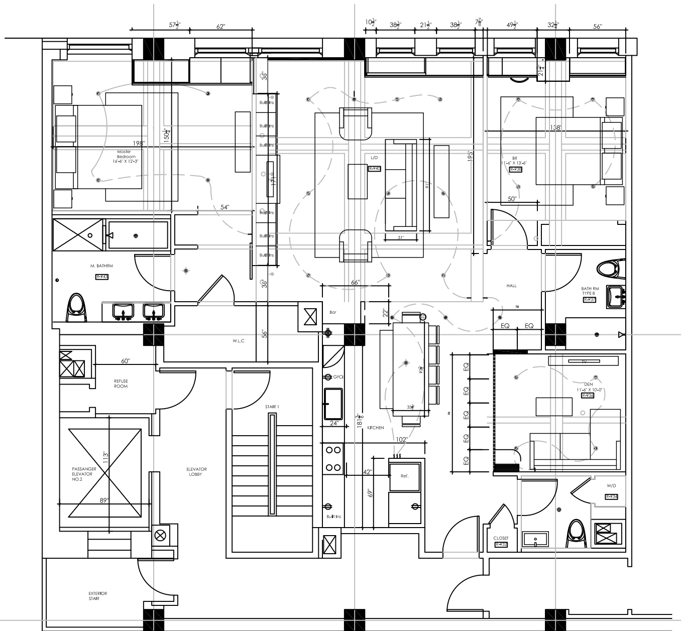
2 Entertainment Furniture Plan Opt 1 Scale: \frac{1}{8} " = 1'-0"
