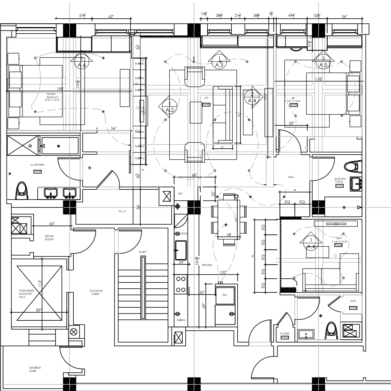
1 Everyday Furniture Plan Opt 1 Scale: \frac{1}{8} " = 1'-0"
