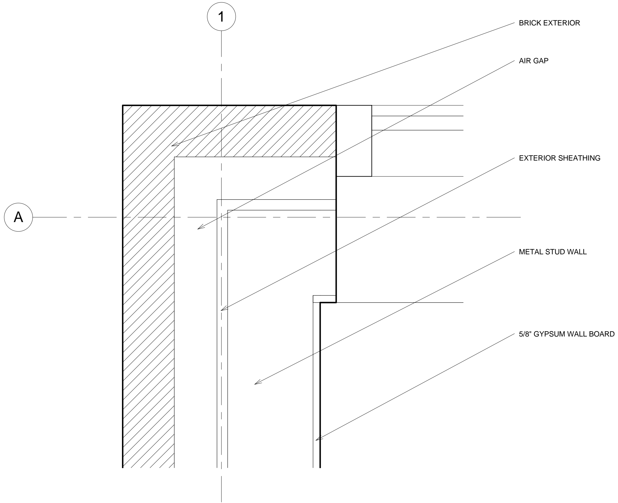
1 Wall Detail 3" = 1'-0"
