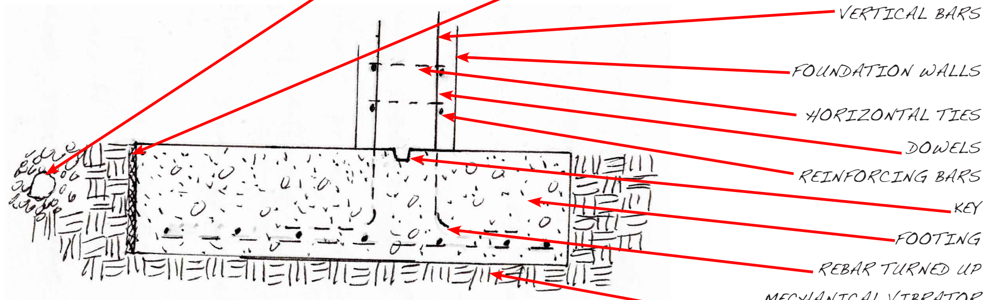
Analysis Sketch of Process for Pouring Foundation
