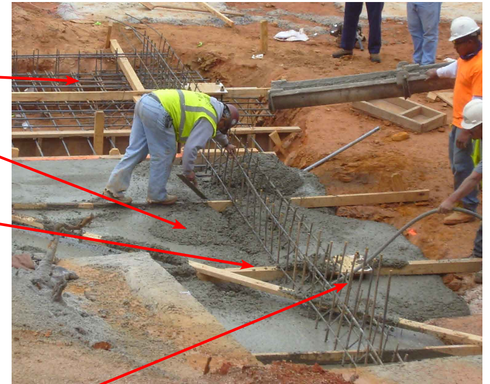
Observation of Form Liners and bracing
