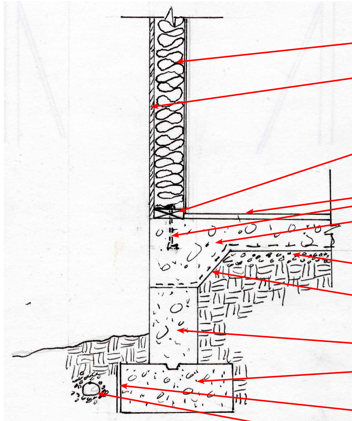
Anaylsis Sketch of Partial Wall Section
