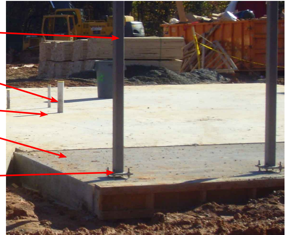
Observation of Foundation and Columns for Gable
