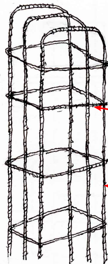
Observation Sketch of Reinforcement Preparation for Column
