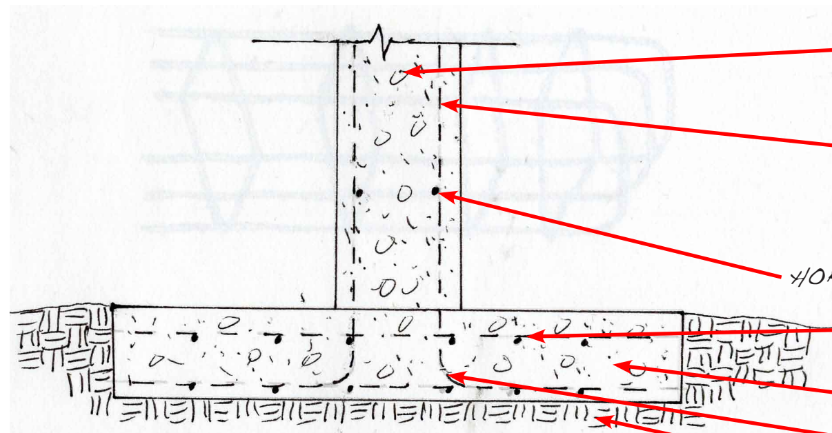
Analysis Sketch of Partial Wall Section
