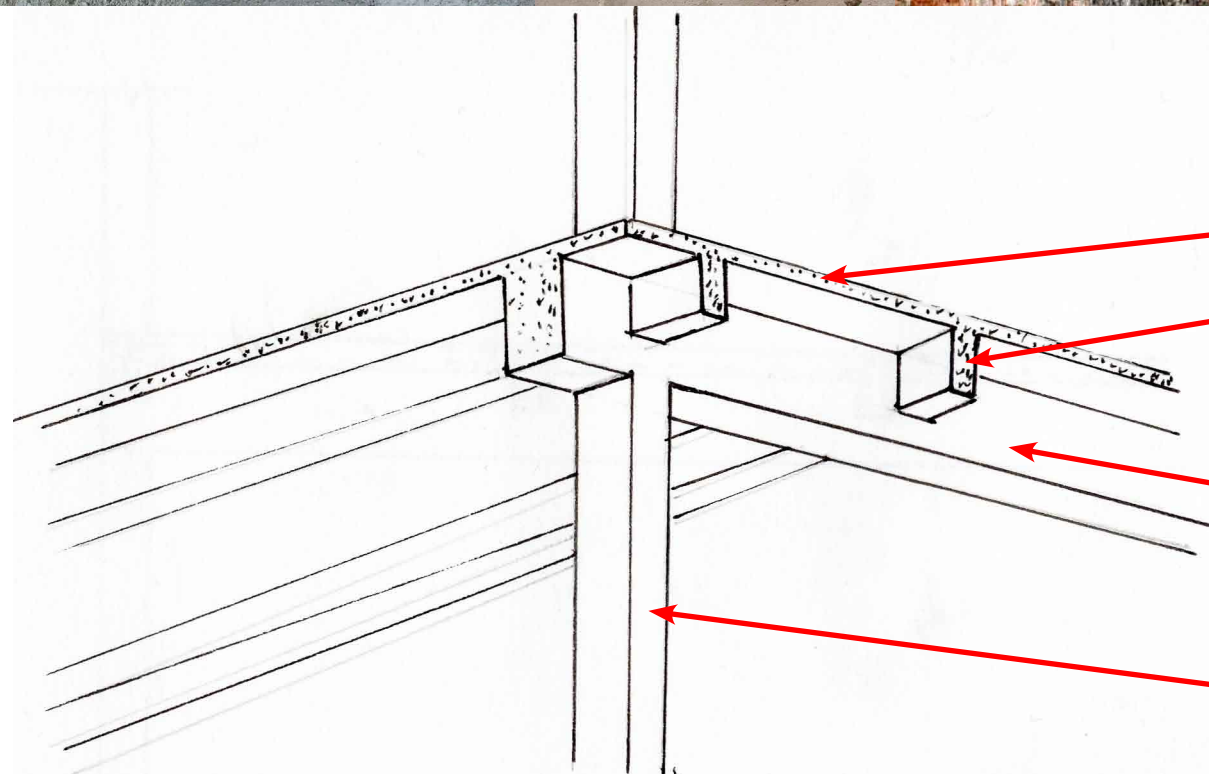
Analysis Sketch of One Way Slab and Beam Floor
