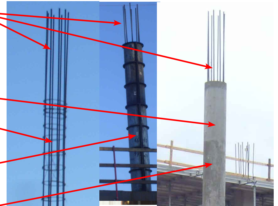
Observation of Round Column Construction Process
