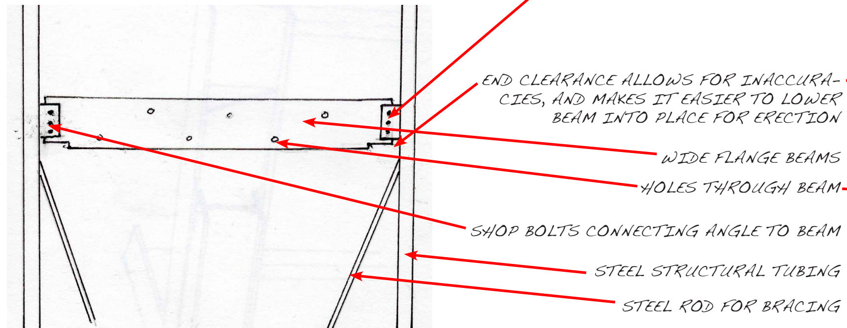
Documented Sketch of Steel Construction
