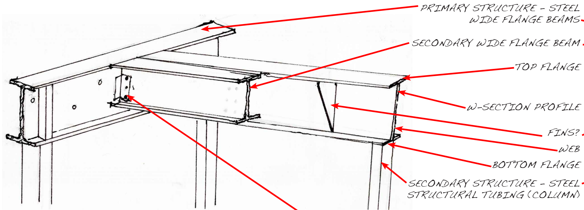
Documented Sketch of Steel Construction
