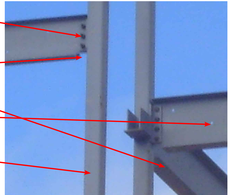
Observation of Primary & Secondary Connections
