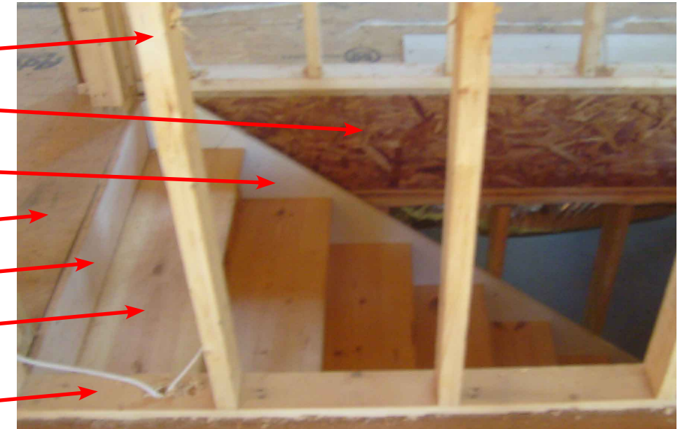
Observation of Stair Components into basement area and framing out of floor area around it
