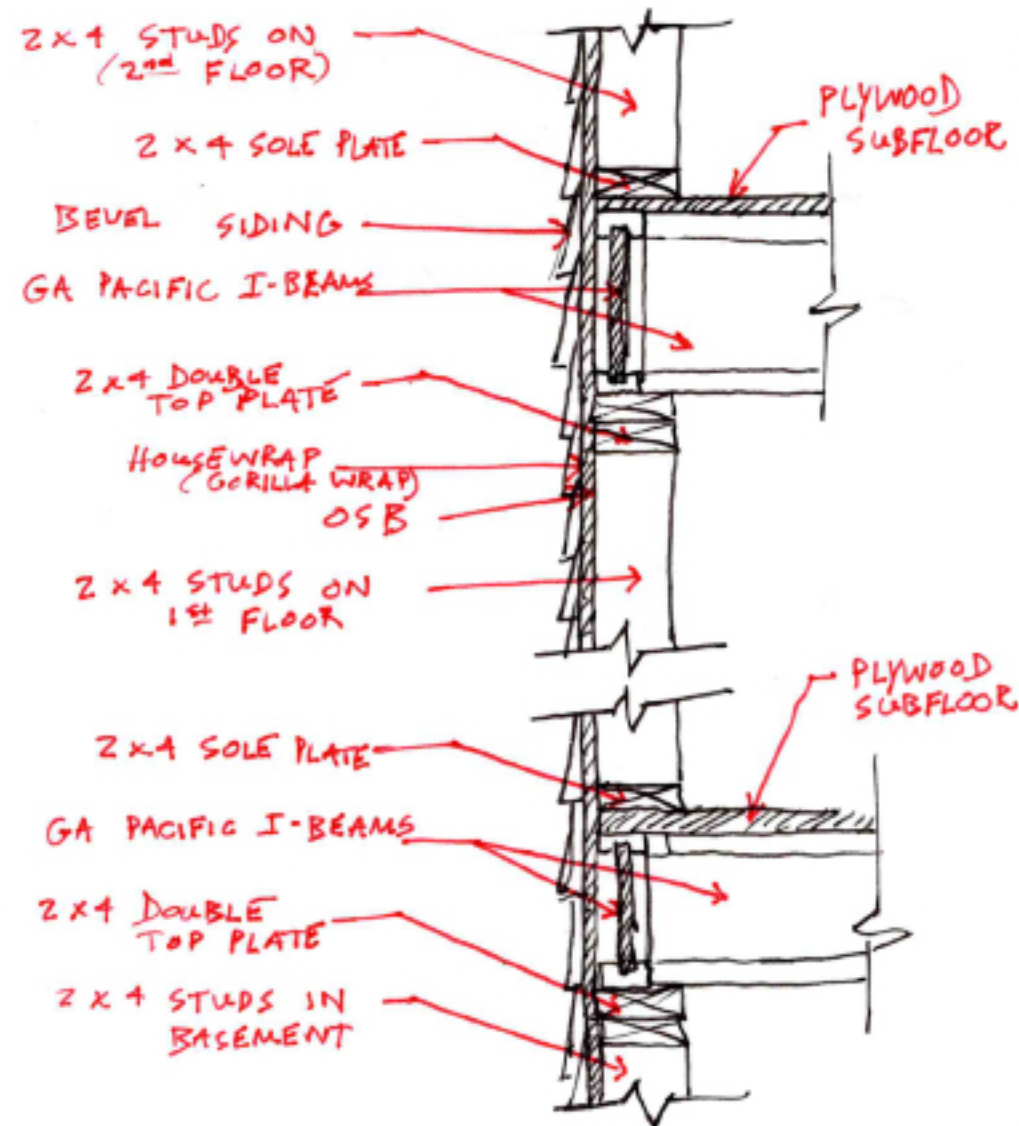
Analysis of Platform Framing Construction
