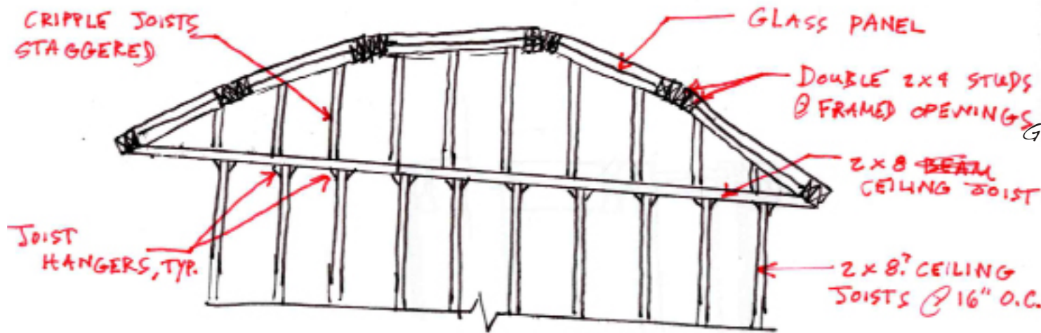
Observation of Framing Layout above Bow Window
