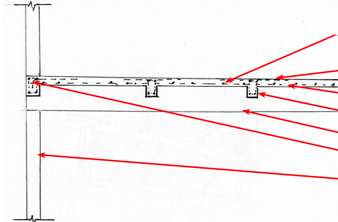
Analysis Sketch of Section through One Way Slab and Beam Floor
