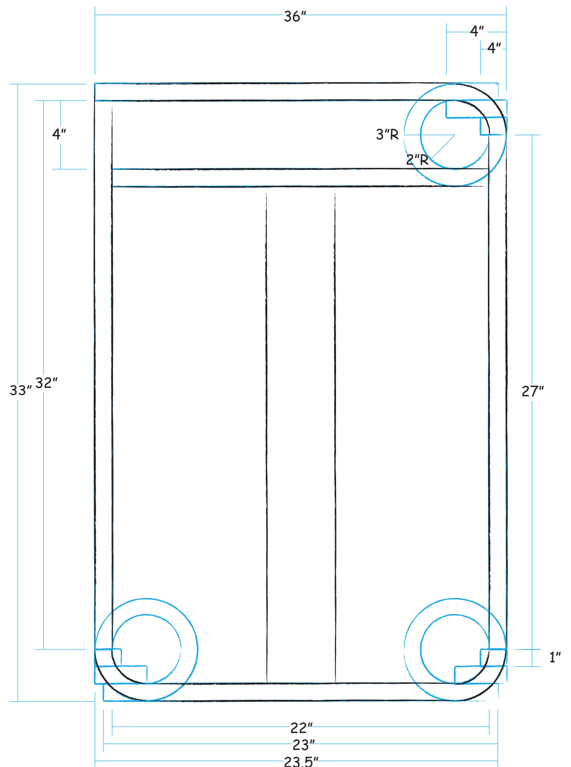
SIDE VIEW
