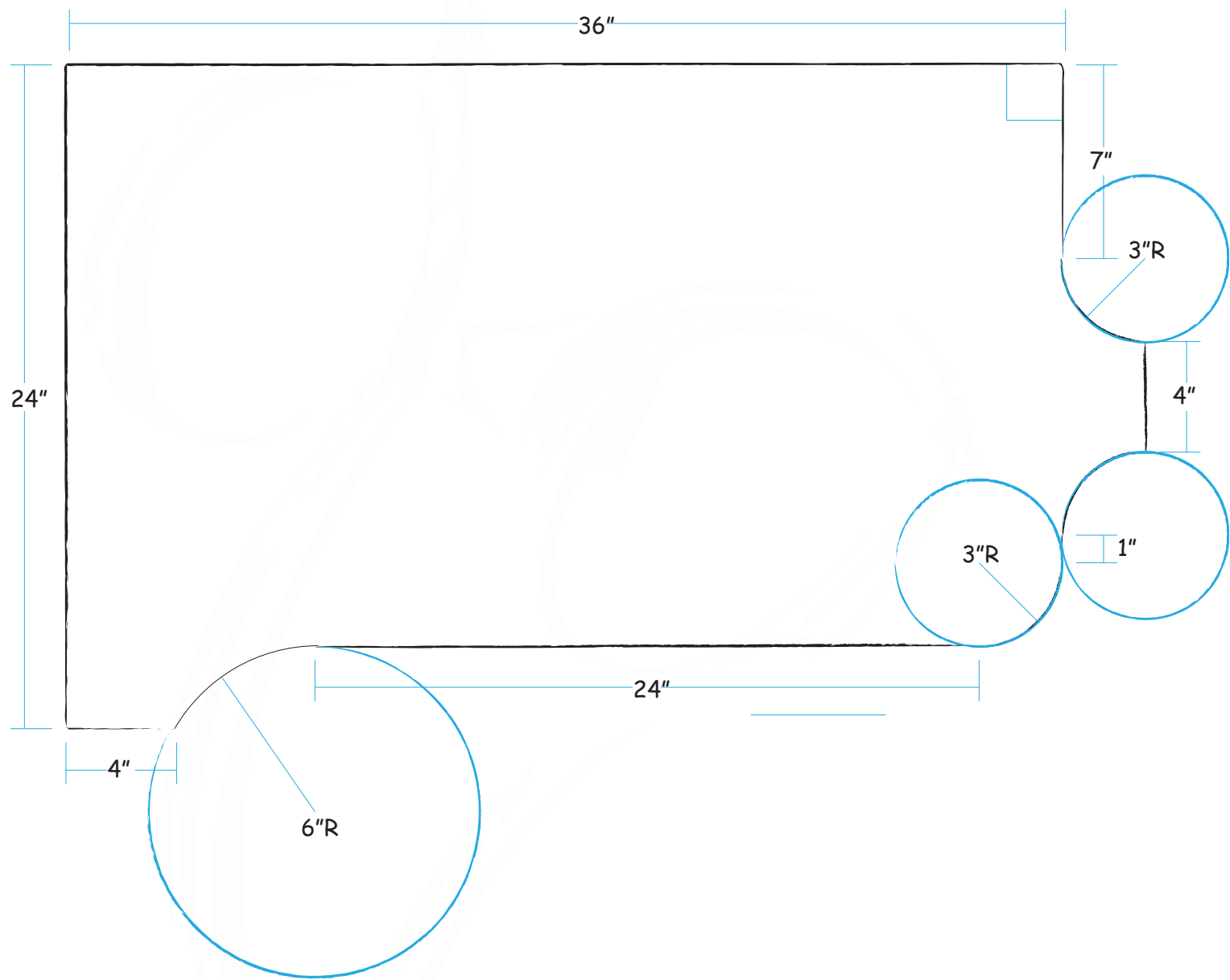
TOP VIEW
