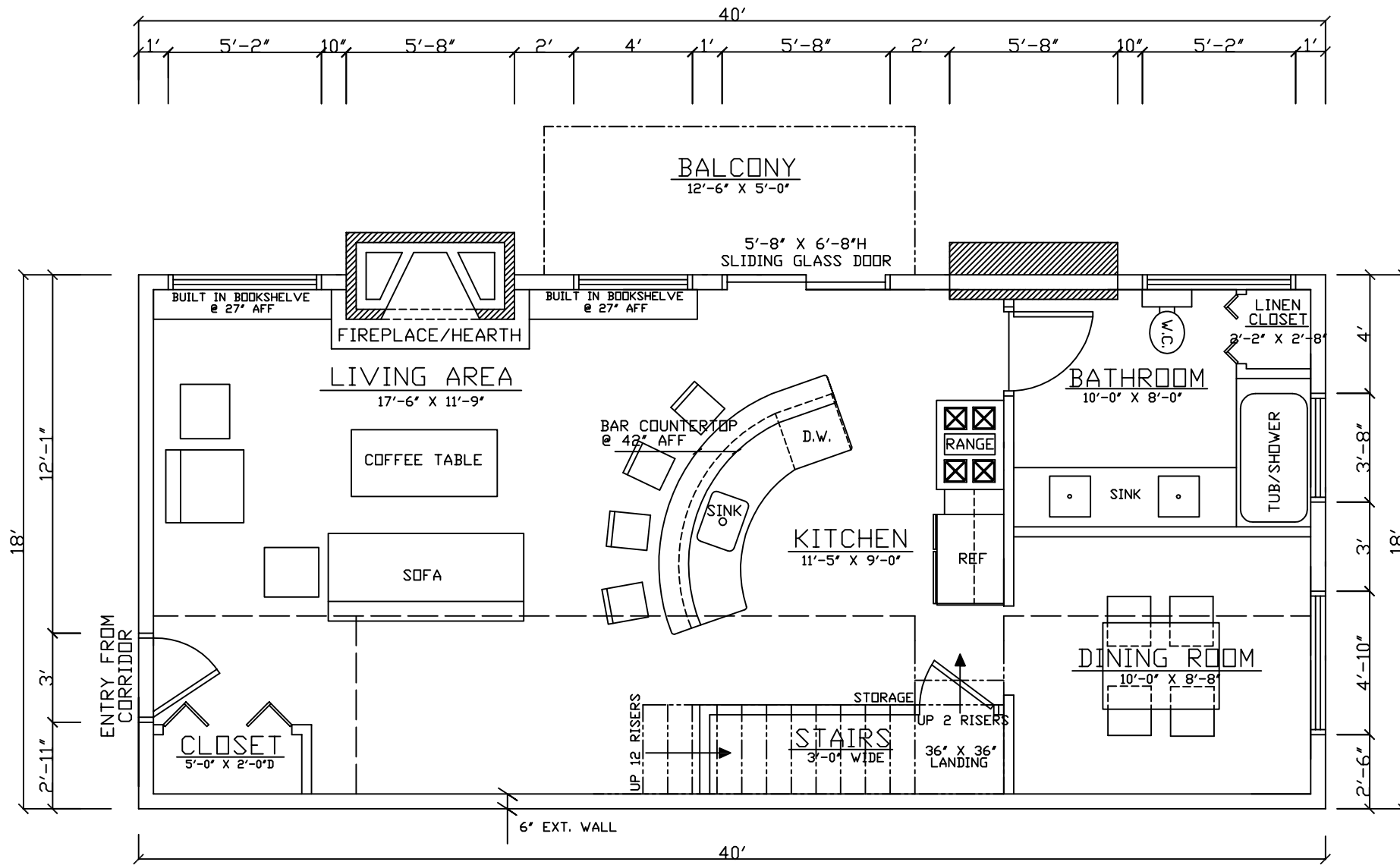
PROPOSED FLOOR PLAN-FIRST FLOOR
