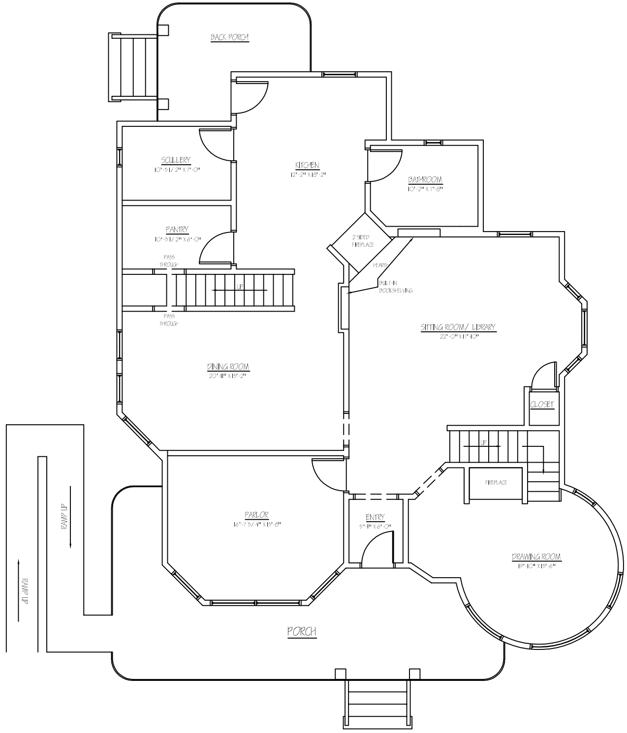
PROPOSED FIRST FLOOR PLAN SCALE: 1/4" = 1'-0"
